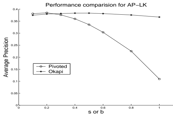
Figure 2: Performance Comparison between Okapi and Pivoted for AP-LK.
