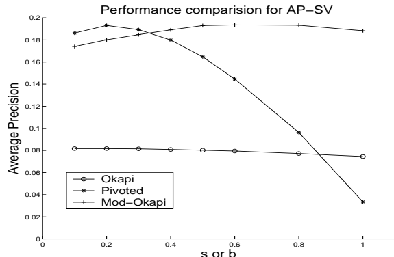
Figure 4: Performance Comparison between modified Okapi, Okapi and Pivoted for AP-SV.
