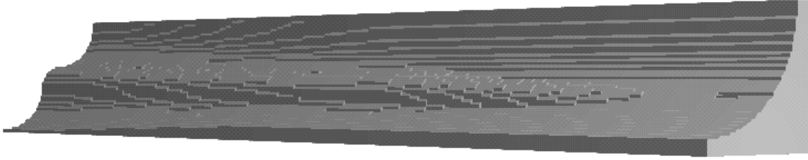
Figure 2. One fourth the quatrefoil to circular taper, shown in perspective (MAFIA simulation).
