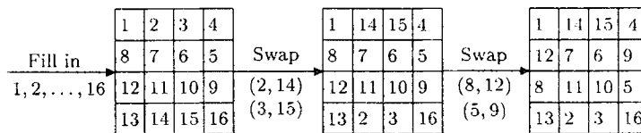
Fig.6. 4 \times 4 magic square produced by the deterministic program. (p.349)
