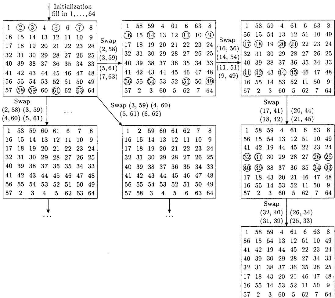
Fig.7. 8 \times 8 magic squares produced by the non-deterministic program. (p.349)
