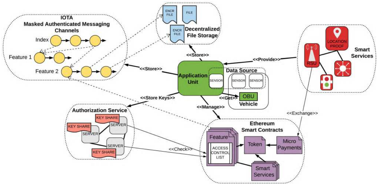
FIGURE 4. System architecture.
