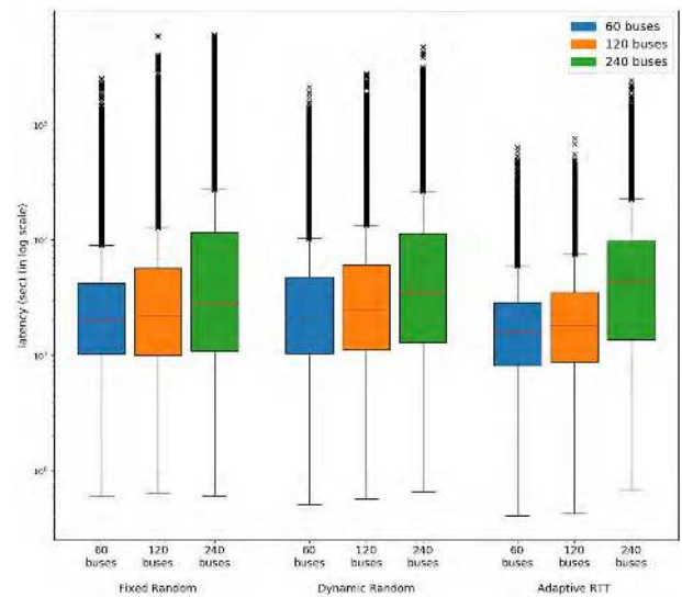
FIGURE 10. Latency (in log scale): boxplots for tests with 60, 120, 240 buses.
