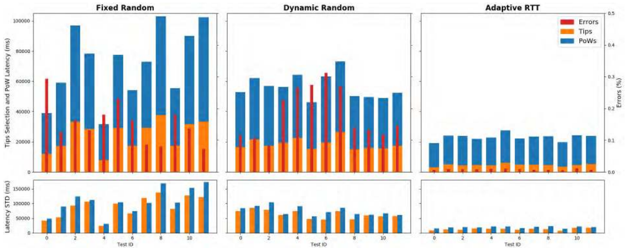
FIGURE 9. 60 bus tests: average latencies, standard deviation and errors for the three different schemes (lower is better).
