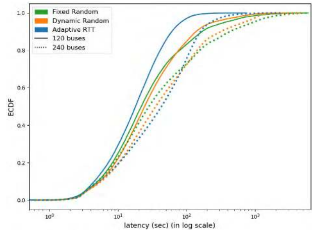
FIGURE 12. Empirical cumulative distribution function for tests with 120 and 240 buses.
