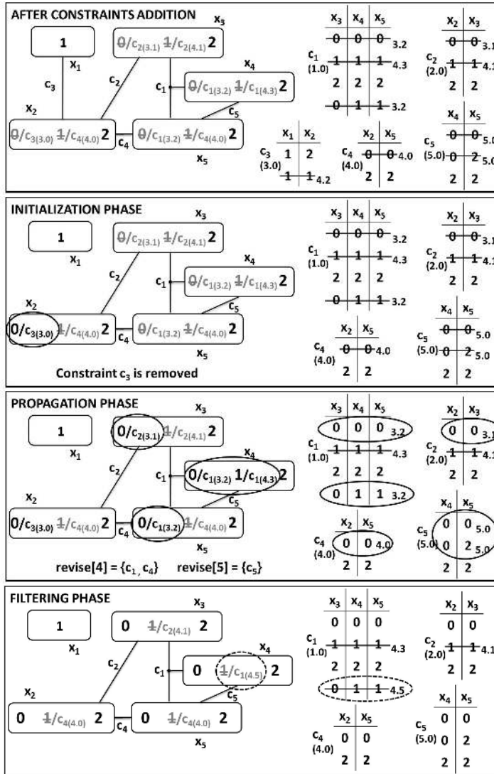
Figure 8.1: Removing constraint c3 in the CSP example from Figure 1. Associated timestamps are written as “3.1” for (dp = 3, lt = 1) next to each added constraint and removed tuple. Justifications (constraint and time) are also shown next to each deleted value. Plain circles show the values and tuples restored since the previous phase, while dashed circles represent values and tuples re-filtered.
