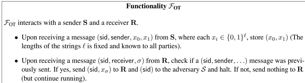
Figure 2: The oblivious transfer functionality \mathcal{F}_{\text{OT}} [CLOS02].
