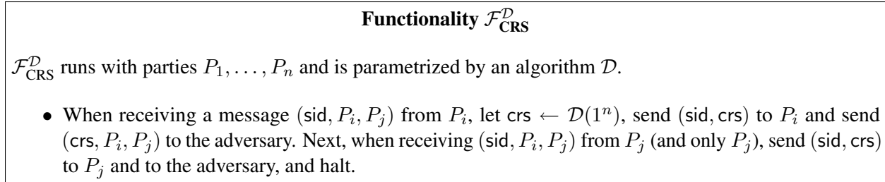
Figure 1: The common reference string functionality \mathcal{F}_{\text{CRS}}^{\mathcal{D}} [CR03].
