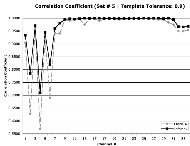
Figure 4 Correlation between original & ICA-filtered data across the 34 electrodes.
