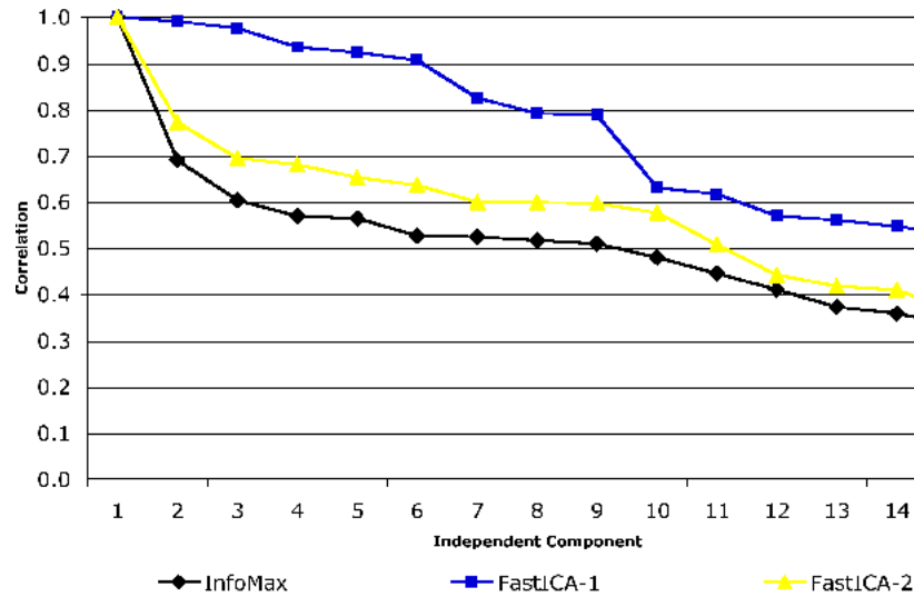
Figure 5 Correlation between original and ICA-filtered data across the 34 electrodes.
