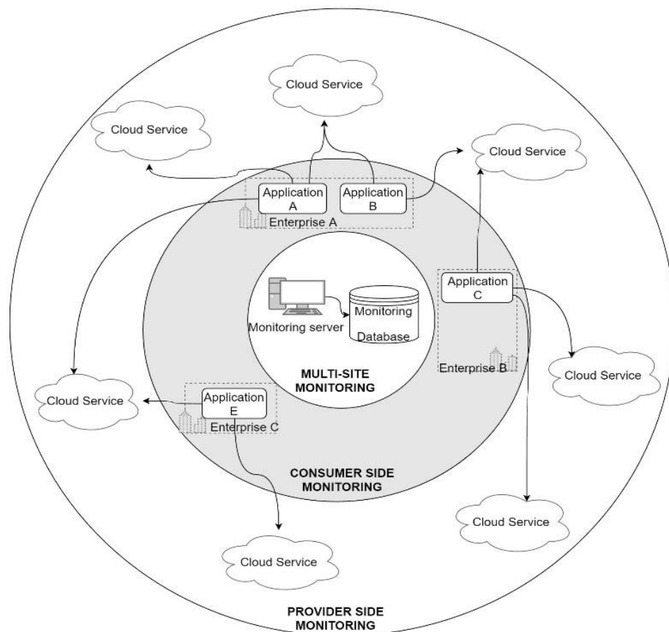
Figure 7.2. Multi-site cloud service monitoring
