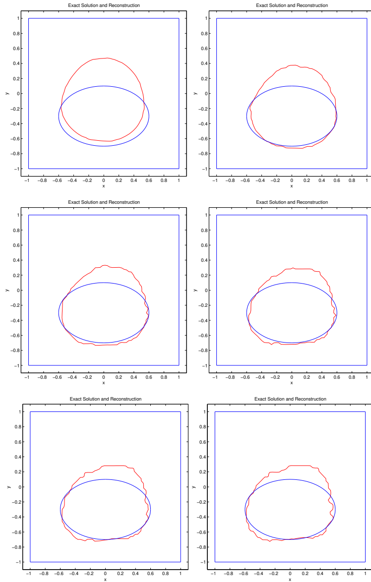
FIG. 6. Reconstructions with the Stefan-type flow at iterations 50, 100, 150, 200, 250 and 300.
