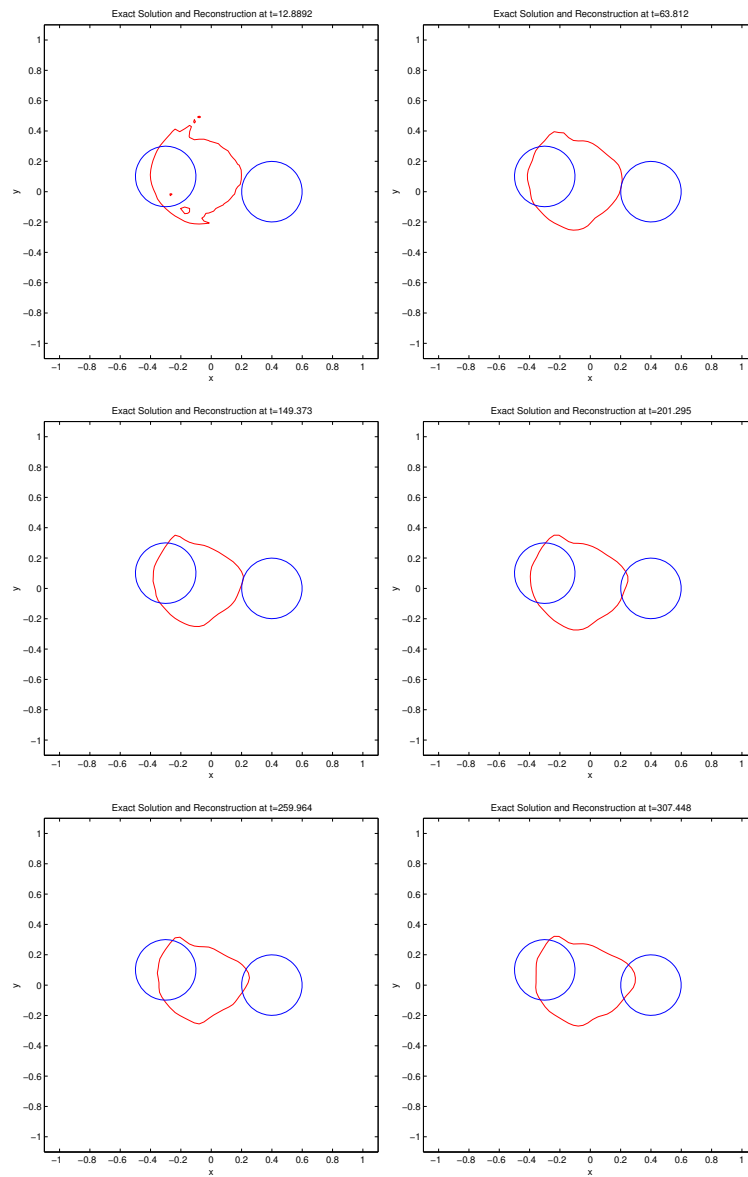
FIG. 3. Reconstructions with the Stefan-type flow at iterations 25, 50, 75, 100, 125 and 150.
