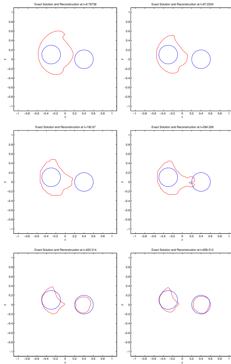
FIG. 1. Reconstructions with the Hadamard flow at iterations 25, 50, 75, 100, 125 and 150.
