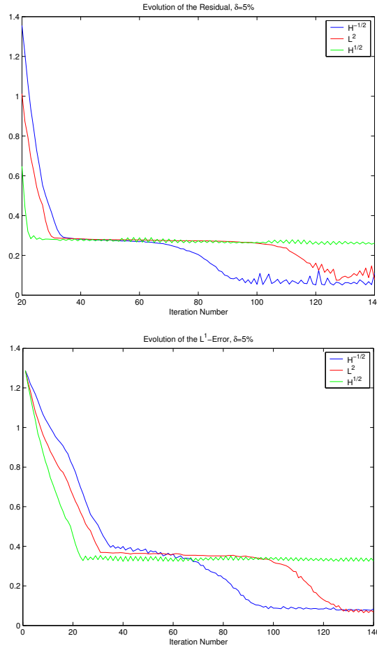
FIG. 4. Evolution of the residual (top) and error in the L^1 -norm (bottom) during exact solution and reconstructed shape for \delta = 5\% noise.
