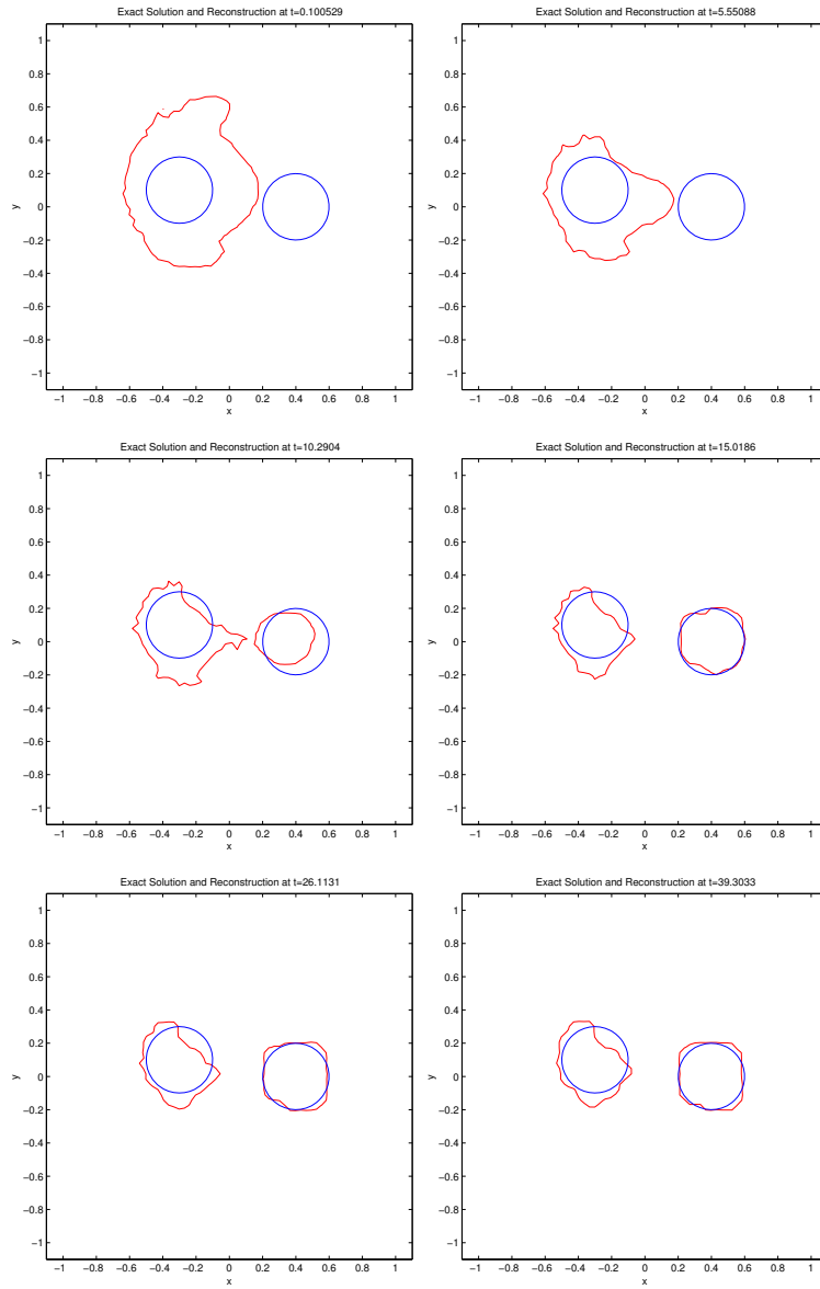
FIG. 2. Reconstructions with the Mullins–Sekerka flow at iterations 25, 50, 75, 100, 125 and 150.
