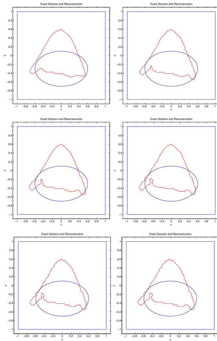
FIG. 5. Reconstructions with the Hadamard flow at iterations 50, 100, 150, 200, 250 and 300.
