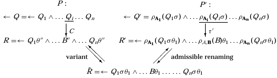
Fig. 5. Illustrating the proof of Theorem 8.2.
