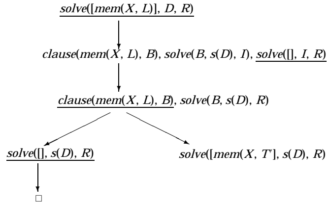
Fig. 1. Incomplete SLD-tree for Example 2.5.
