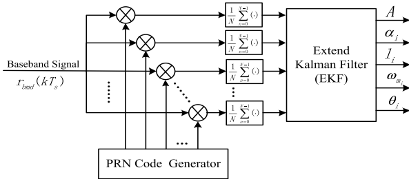
FIGURE 10. Multipath-doppler parameters estimator.
