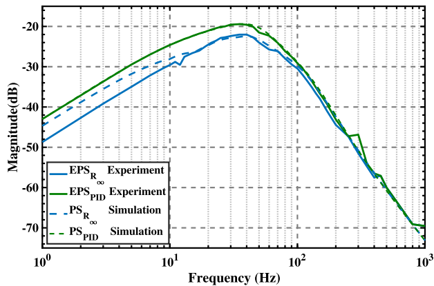
FIGURE 13. The process pseudo-sensitivity and process sensitivity of the system with the CgLp and PID controllers which are deduced experimentally, EPS_{R_{\infty}} and EPS_{PID} are practical process sensitivity of the system with the controller C_R and C_{PID} , respectively.
