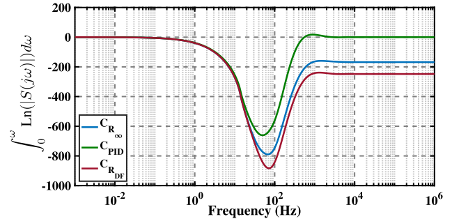
FIGURE 8. The magnitude of the integral of the sensitivity versus frequency.
