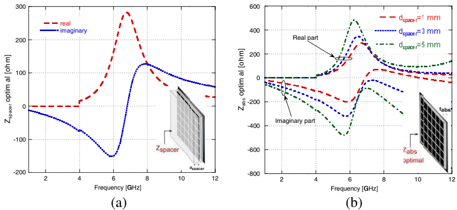
Figure 5. Optimal input impedances at two different interfaces of the multilayer for achieving perfect reflection up to 4 GHz and complete reflection after 4 GHz at the input of the system: (a) Real and imaginary parts of the optimal input impedance before the foam spacer. (b) Real and imaginary parts of the optimal impedance at the input of the loading absorber for different values of the foam spacer.
