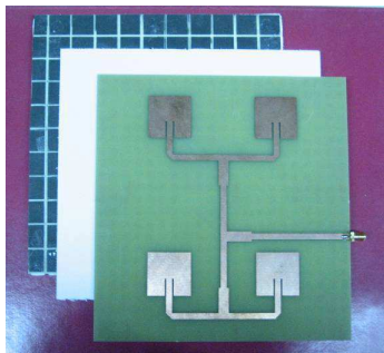
Figure 10. A picture of the manufactured prototype of the low RCS antenna.
