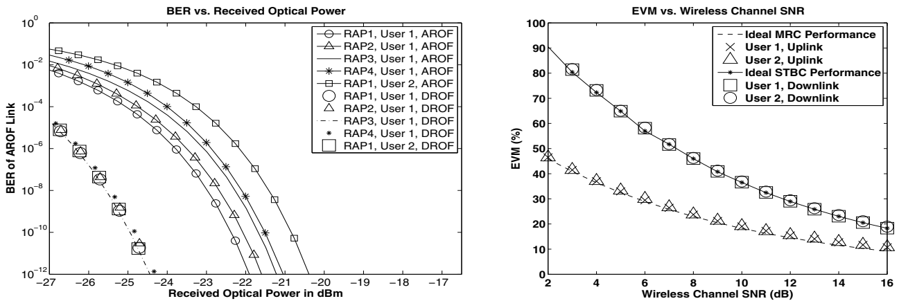
(a) BER performance of the AROF and DROF links.
