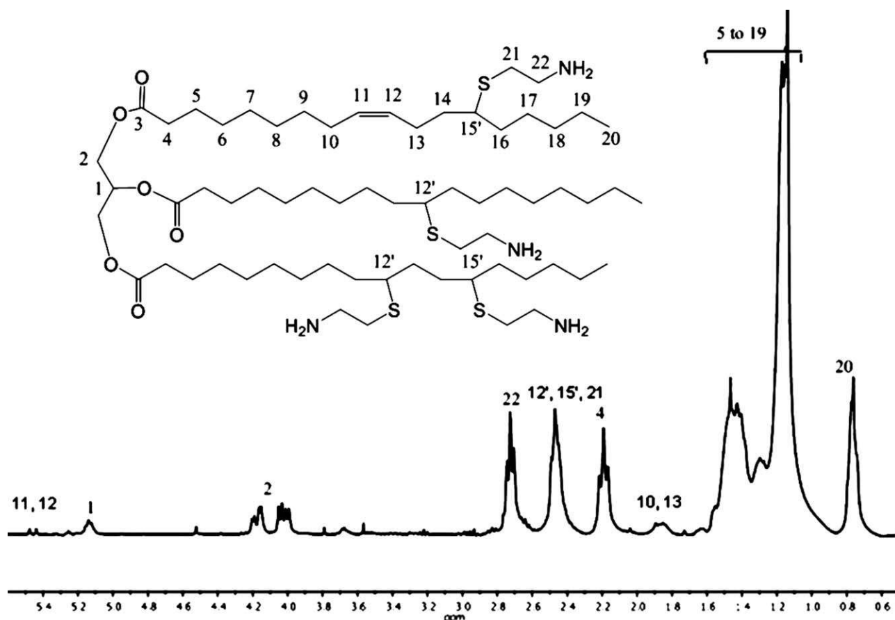
FIGURE 2 ^1\text{H} NMR spectrum of AGSO in \text{CDCl}_3 .
