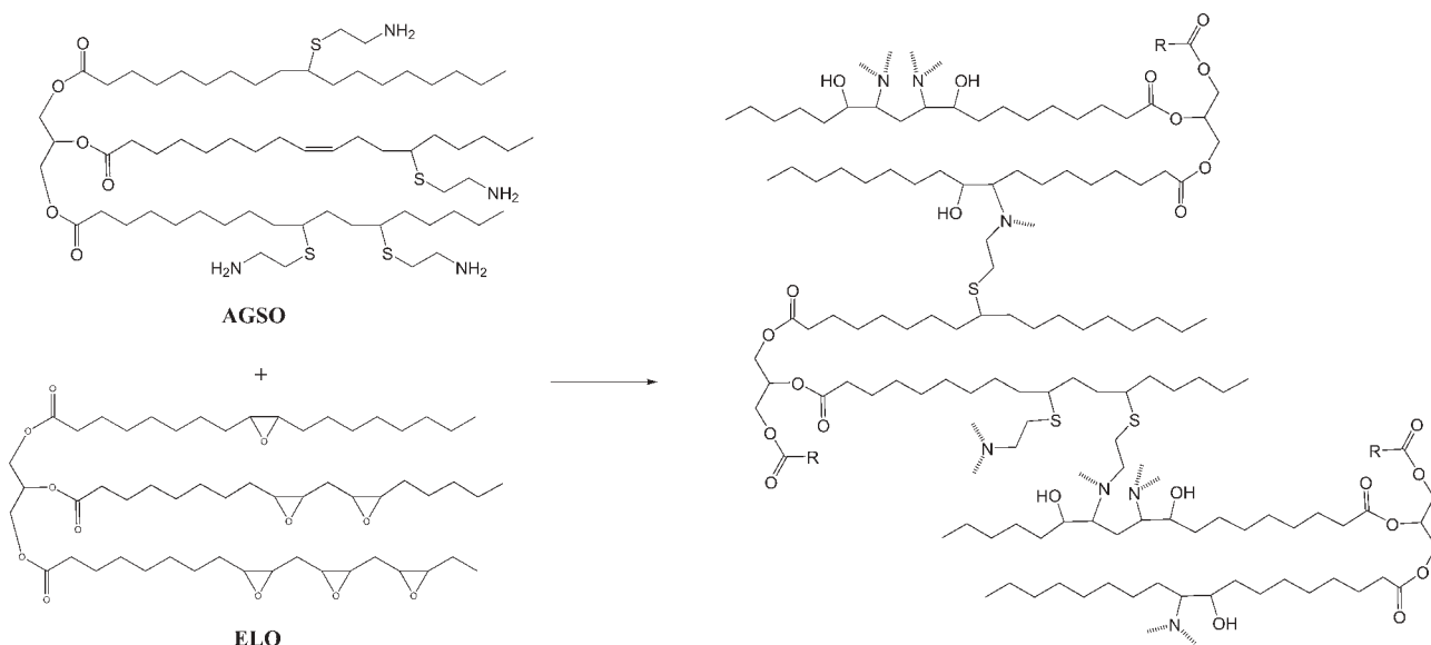
SCHEME 2 Crosslinking reaction between ELO and AGSO.
