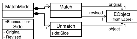
Figure 18 Match Metamodel
