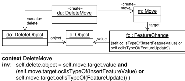
Figure 27 Delete-Move Conflict
