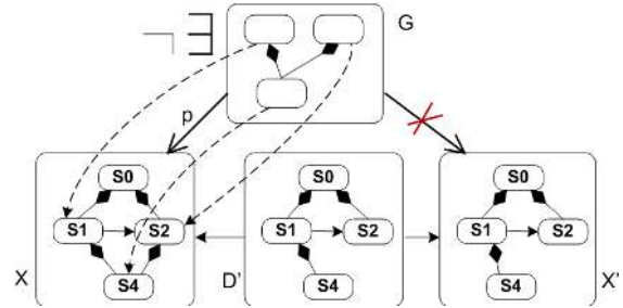
Figure 14 Repair action for a negative constraint
