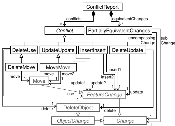
Figure 24 Conflict Metamodel
