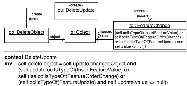
Figure 28 Delete-Update Conflict
