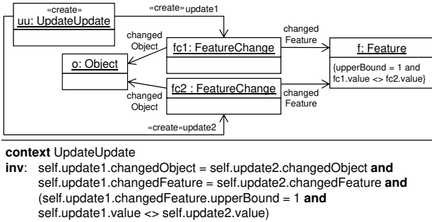
Figure 29 Update-Update Conflict
