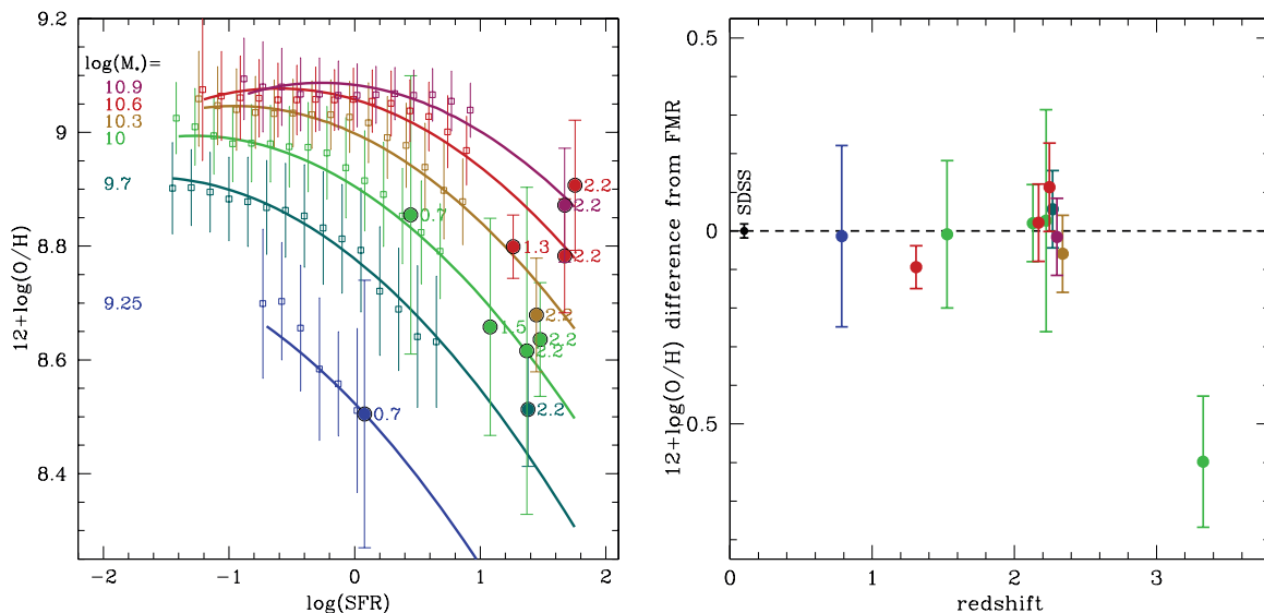
Figure 4. Left-hand panel: metallicity as a function of SFR for galaxies in the bins of M_* containing high-redshift galaxies. The values of \log(M_*) are shown by the labels on the left-hand side. Empty square dots are the median values of metallicity of local SDSS galaxies, with error bars showing 1\sigma dispersions. Lines are the fits to these data. Solid dots are median values for high-redshift galaxies with z < 2.5 in the same mass bins, with labels showing redshifts. Right-hand panel: metallicity difference from the FMR for galaxies at different redshifts, colour-coded in mass as in the left-hand panel. The SDSS galaxies defining the relation are showing at z \sim 0.1 with their dispersion around the FMR. All the galaxy samples up to z = 2.5 are consistent with no evolution of the FMR defined locally. Metallicities lower by \sim 0.6 dex are observed at z \sim 3.3 .
