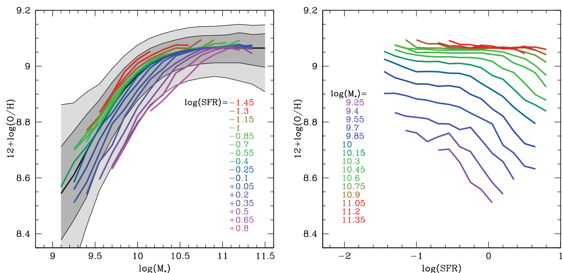
Figure 1. Left-hand panel: the mass–metallicity relation of local SDSS galaxies. The grey-shaded areas contain 64 and 90 per cent of all SDSS galaxies, with the thick central line showing the median relation. The coloured lines show the median metallicities, as a function of M_* , of SDSS galaxies with different values of SFR. Right-hand panel: median metallicity as a function of SFR for galaxies of different M_* . At all M_* with \log(M_*) < 10.7 , metallicity decreases with increasing SFR at constant mass.
