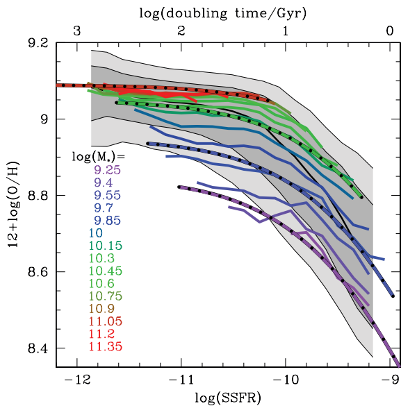
Figure 6. Metallicity of SDSS galaxies as a function of SSFR. The grey-shaded areas contain 64 and 90 per cent of all SDSS galaxies, with the thick central line showing the median relation. The coloured lines show the median metallicities for different values of M_* . The lines with black dots show fits to these metallicity distribution for four values of \log(M_*) , 9.4, 9.7, 10 and 10.9. The model is described in Section 7.1 and includes only dilution for infalling gas and the SK law.
