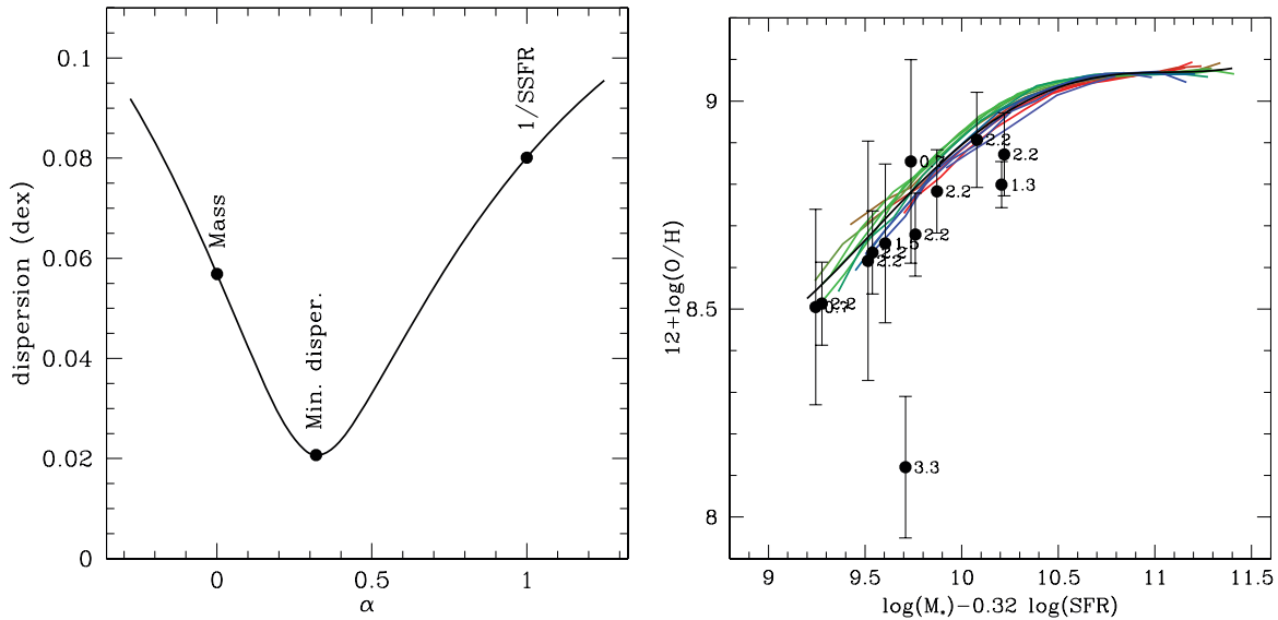
Figure 5. Left-hand panel: residual dispersion of the median values of metallicity of SDSS galaxies as a function of \alpha as defined in equation (3). The values corresponding to the minimum dispersion ( \alpha = 0.32 ), to \alpha = 0 [ \mu_\alpha = \log(M_*) ] and to \alpha = 1 [ \mu_\alpha = -\log(\text{SSFR}) ] are shown. Right-hand panel: metallicity as a function of \mu_{0.32} , which minimizes the residual scatter. Coloured lines are local SDSS galaxies, with colours as in the left-hand panel of Fig. 1. The black line shows the polynomial best fit. Black dots are high-redshift galaxies, labelled with redshifts. These galaxies, except those at z \sim 3.3 , appear to follow the same relation defined by SDSS galaxies.
