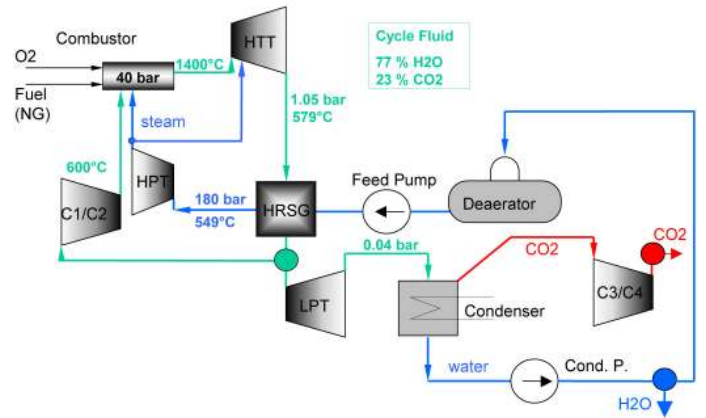
Fig. 1: Principle flow scheme of Graz Cycle power plant
