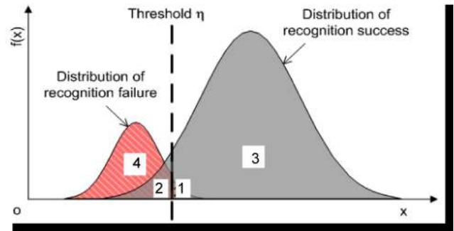
Fig. 1. Thresholding a per datum reliability or “quality” measure to predict recognition system success produces 4 different “cases”, depending on the success of the recognition system on a sample and the reliability-based prediction of success or failure associated with that sample.
