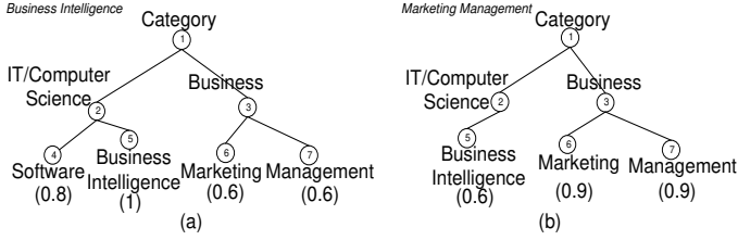
Fig. 3. Two fuzzy category trees of two learning activities: (a) is the fuzzy category tree of the subject Business Intelligence . (b) is the fuzzy category tree of the subject Marketing Management .
