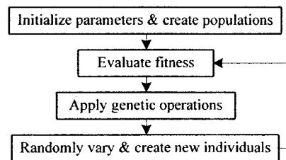
Figure 2.2. Flowchart of evolutionary GP.
