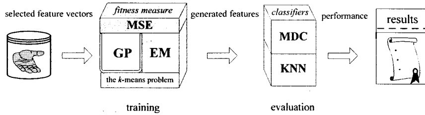
Figure 4.13. The GP-EM-MSE hand-based biometric identification system.
