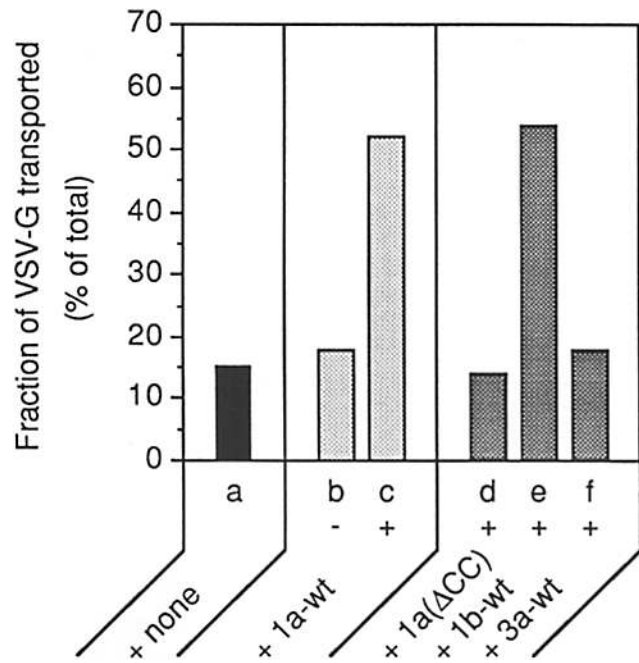
Figure 8. Wild-type rabla and rab1b reverse rabla(S25N) mediated inhibition in vitro and require posttranslational prenylation for function. Perforated NRK cells were incubated in vitro with processed rabla(S25N) alone (lane a) and in combination with equivalent amounts of the indicated proteins (lanes b–f) preincubated in the absence (–; lane b) or presence (+; lanes c–f) of GGPP. Transport was assessed and quantitated as described in the legend to Fig. 8 and in Materials and Methods.
