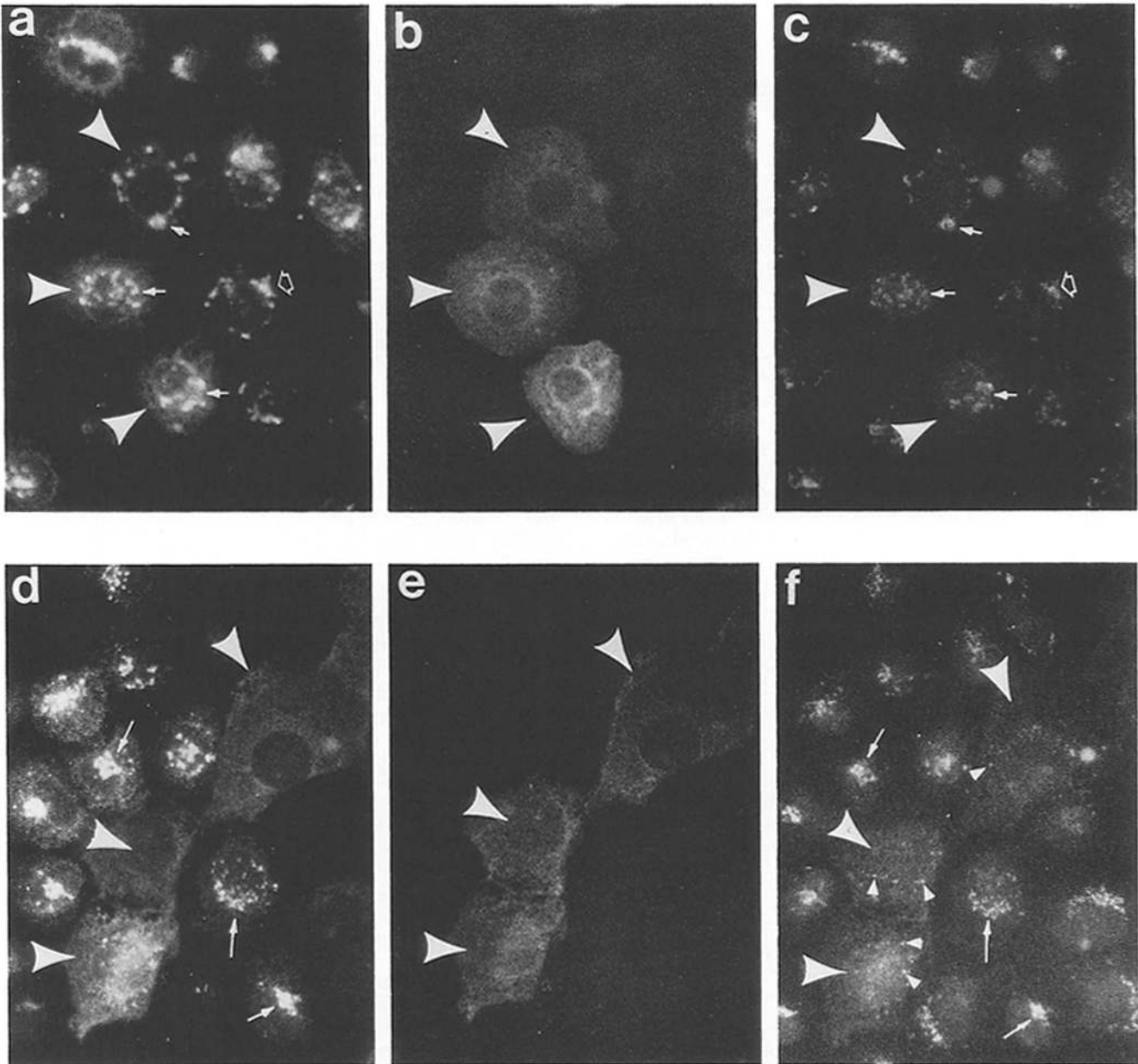
Figure 5. Microinjection of recombinant rabla(S25N) inhibits protein export from the ER and triggers dispersal of the Golgi complex. NRK cells were infected with the ts045 strain of VSV at the restrictive temperature and microinjected with a 10–20-fold excess of recombinant rabla ( a–c ) or rabla(S25N) ( d–f ) over the endogenous rab1 pool in combination with an IgG marker as described in Materials and Methods. After a 1.5-h incubation at the restrictive temperature, the cells were shifted to the permissive temperature for 1.5 h, and the distribution of VSV-G ( a and d ), IgG ( b and e ), and Man II ( c and f ) were determined by indirect immunofluorescence as described in Materials and Methods. The large arrowheads denote the microinjected cells. The small arrows in panels a and c denote colocalization of VSV-G with representative Golgi structures in cells injected with wild-type rabla; the open arrow in panels a and c points to a Golgi structure in a non-injected cell. The arrows in panels d and f indicate Golgi in non-injected cells; the small arrowheads in panel f denote dispersed Golgi fragments in cells injected with the rabla(S25N) mutant.
