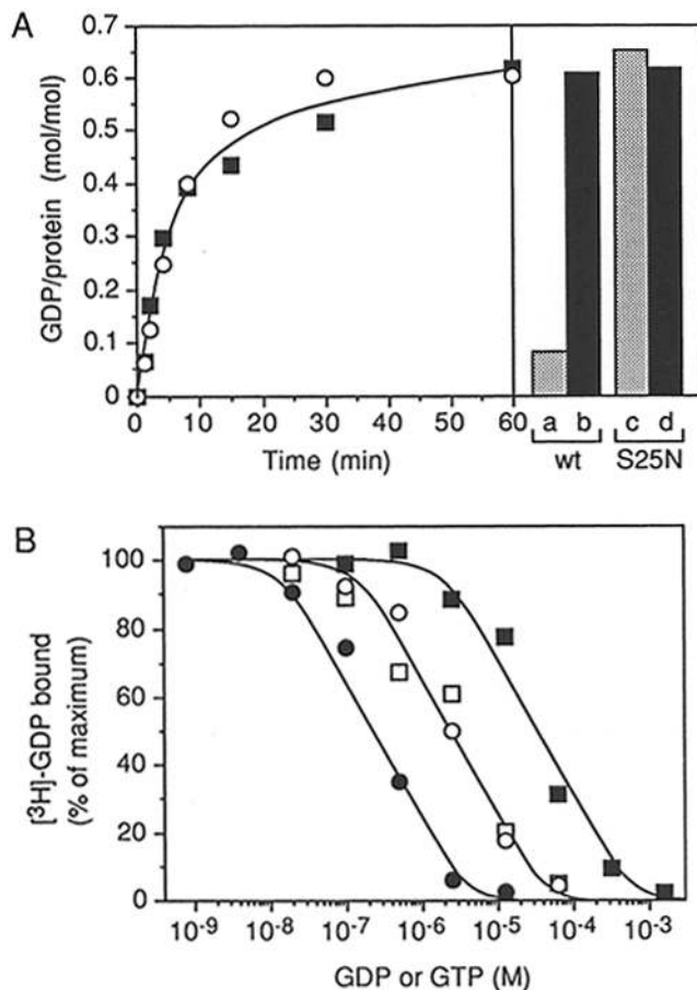
Figure 1. The rabla(S25N) mutant shows preferential affinity for GDP. (A) Time course and Mg 2+ dependence of GDP exchange. Exchange reactions were performed in duplicate by incubating 0.5 \mu g (20 pmol) of recombinant protein at 32°C with 2.5 \mu M [ 3 H]GDP ( \sim 5,000 cpm/pmol) in the presence of EDTA and MgCl 2 . Bound [ 3 H]GDP was quantitated by liquid scintillation counting after capture of the proteins on nitrocellulose membranes as described in Materials and Methods. (Left panel) The wild-type (○) and mutant proteins (■) were incubated for the specified times with [ 3 H]GDP in the presence of 5 mM EDTA and 4.5 mM MgCl 2 , and the amount of protein-bound GDP was determined for each time point. (Right panel) The wild-type (wt, lanes a and b) and mutant proteins (S25N, lanes c and d) were incubated for 1 h with [ 3 H]GDP in the presence of 5 mM EDTA and either 10 mM MgCl 2 (gray bars, lanes a and c) or 4.5 mM MgCl 2 (black bars, lanes b and d), and the amount of protein-bound GDP was determined. (B) Relative affinities of the proteins for GDP and GTP. The wild-type (○, ●) and mutant (□, ■) proteins were incubated for 1 h with [ 3 H]GDP in the presence of 5 mM EDTA and 4.5 mM MgCl 2 , and the indicated concentrations of unlabeled GDP (○, □) or GTP (●, ■). The results are expressed as the percentage of the amount of [ 3 H]GDP bound in the absence of additional nucleotide.
