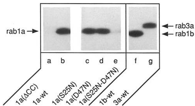
Figure 6. Recombinant rabla(S25N) can be posttranslationally prenylated in vitro. 1 \mu g (40 pmol) of the indicated recombinant wild-type and mutant proteins were incubated for 1 h at 32°C in the presence of rat liver cytosol, ATP, and 0.52 mM [ ^3 H]GGPP (19.3 Ci/mmol) as described in Materials and Methods. The samples were analyzed by SDS-PAGE and fluorography.
