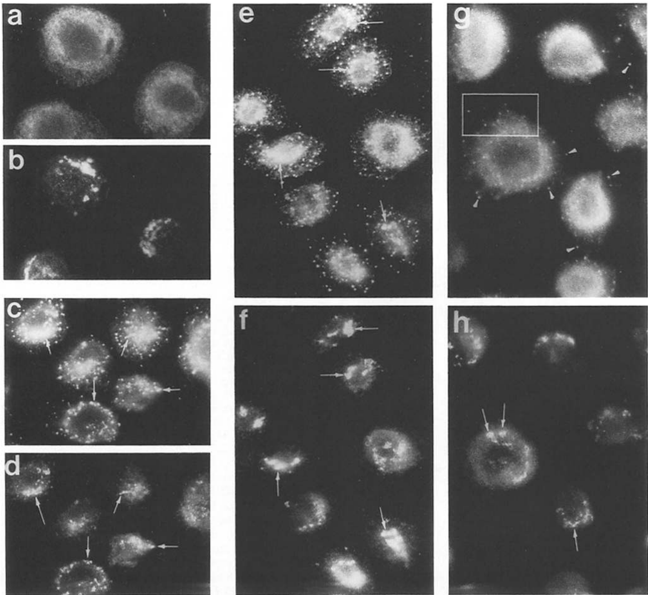
Figure 9. The rab1a(S25N) mutant prevents export of VSV-G from the ER in vitro. NRK cells were infected with the ts045 strain of VSV at the restrictive temperature, permeabilized with digitonin, and incubated in the presence of cytosol and ATP for 30 min on ice ( a and b ) or at 32°C ( c-h ) as described in the Materials and Methods. The reactions contained no additions ( a-d ) or were supplemented with posttranslationally processed wild-type rab1a ( e and f ) or rab1a(S25N) ( g and h ). The distribution of VSV-G ( a , c , e , and g ) or Man II ( b , d , f , and h ) was determined by indirect immunofluorescence as described in Materials and Methods. The arrows in panels c and d or e and f denote colocalization of VSV-G with Man II. In the presence of the rab1a(S25N) mutant VSV-G is largely retained in the ER ( g ) and is absent from the Golgi structures ( arrows in h ). The box and arrowheads in panel g illustrate markedly reduced formation of VSV-G containing preGolgi intermediates in the presence of the S25N mutant.
