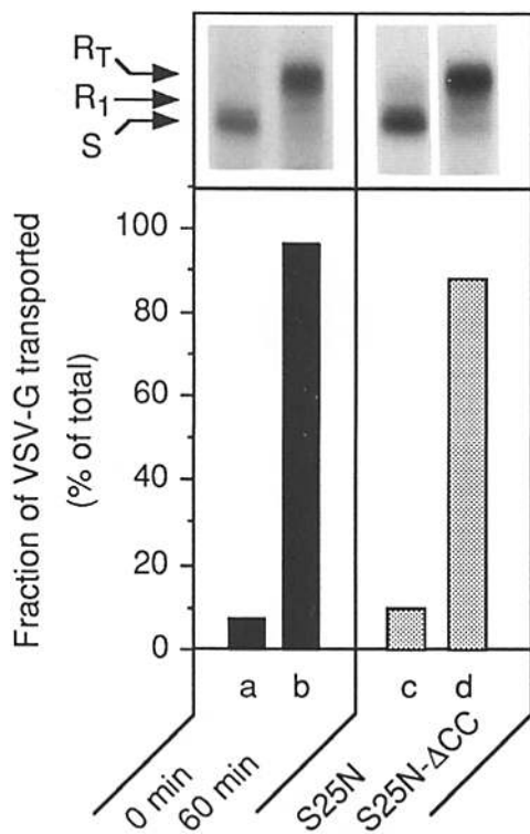
Figure 2. The S25N mutant requires prenylation for function in vivo. HeLa cells were infected with the T7 RNA polymerase-recombinant vaccinia virus vTF7-3 and cotransfected with plasmids encoding VSV-G (lanes a and b ) and the indicated rabla constructs (lanes c and d ) as described in Materials and Methods. After 5 h, cells were pulse-labeled with Trans 35 S-label for 10 min (lane a ), chased for 60 min (lanes b – d ), VSV-G was immunoprecipitated, digested with endo H, and the endo H-sensitive ( S ), the endo H-resistant intermediate ( R I ) and the terminally glycosylated ( R T ) forms were separated by SDS-PAGE, and autoradiographs ( upper panel ) quantitated by scanning densitometry as described in Materials and Methods ( lower panel ). Transport is expressed as the percentage of total VSV-G converted to endo H-resistant forms.
