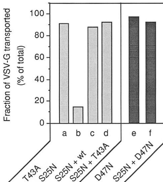
Figure 4. Analysis of effector domain substitutions. The specified rabla single-mutants (lanes a , b , and e ) and combinations of mutant and wild-type ( wt ) proteins ( c , d , and f ) were transiently expressed in HeLa cells. Their effects on transport of VSV-G between the ER and the Golgi compartments were quantitated as outlined in the legend to Fig. 2 and in Materials and Methods. The transport phenotypes of cells expressing the T43A and D47N effector domain mutants alone are illustrated in lanes a and e , respectively. The ability of wild-type rabla, and the T43A or D47N mutants to antagonize S25N inhibition is shown in lanes c , d , and f , respectively.
