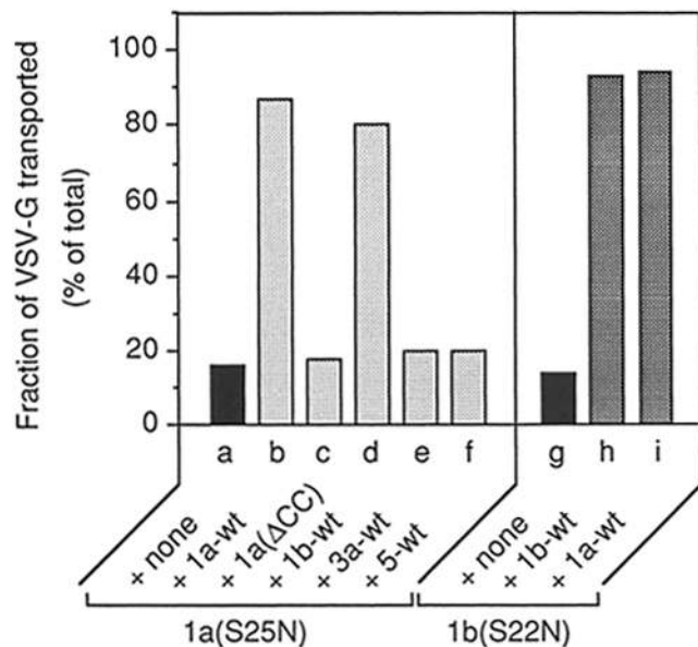
Figure 3. Rabla and rab1b isoforms reverse inhibition of the S25N mutant in vivo. The rabla(S25N) and rab1b(S22N) mutants were transiently expressed in HeLa cells alone (lanes a and g ) or in combination with the indicated mutant or wild-type ( wt ) rab proteins (lanes b – f , h and i ). Their effects on transport of VSV-G between the ER and the Golgi compartments were quantitated as outlined in the legend to Fig. 2 and in the Materials and Methods. Lanes b and c contrast the abilities of wild-type rabla (lane b ) or rabla(ΔCC) (lane c ) to antagonize the inhibitory phenotype of the S25N mutant (lane a ). Lane d shows the consequence of coexpressing the mutant protein with wild-type rab1b. The results of the reciprocal experiments using the analogous rab1b(S22N) mutant are illustrated in lanes g – i .
