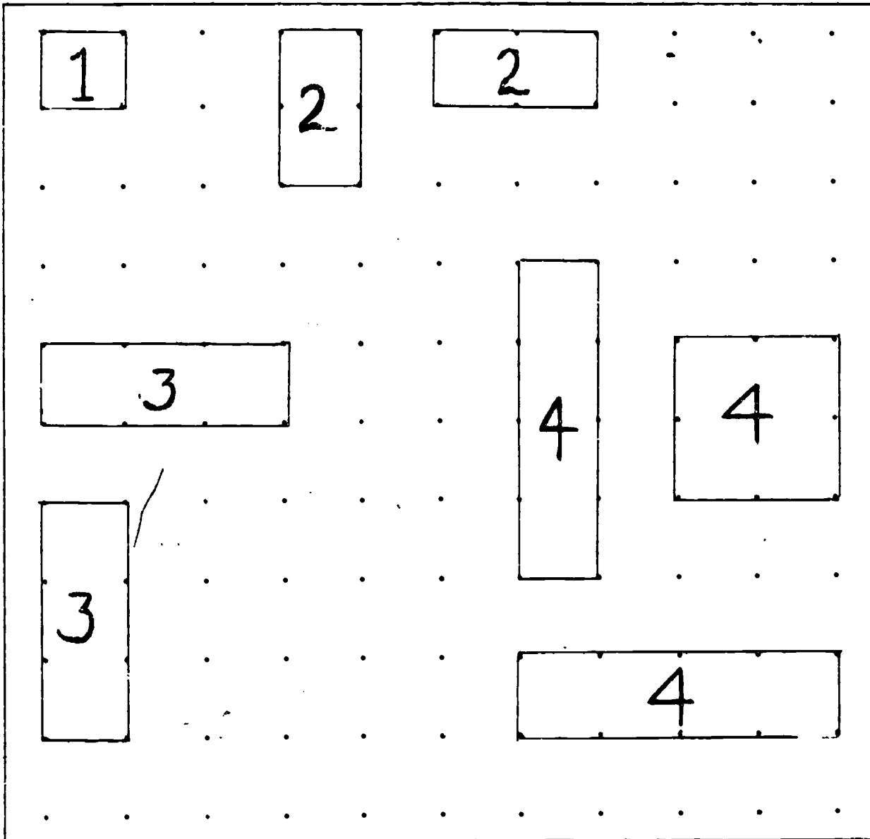
Figure 2. Geoboard illustrating all rectangles of area 1,2,3, and 4.
