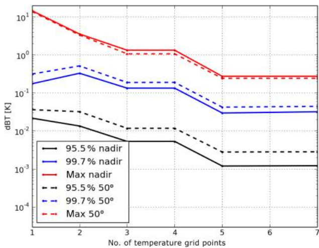
Figure 6. Error statistics of ISMAR observation simulations, given as a function of the temperature grid length used to represent ice hydrometeor scattering properties. The error (dB T) is estimated by comparison to reference calculations. The lines refer to the 95.5 % percentile, the 99.7 % percentile and the maximum value of the errors, for two different observation directions.
