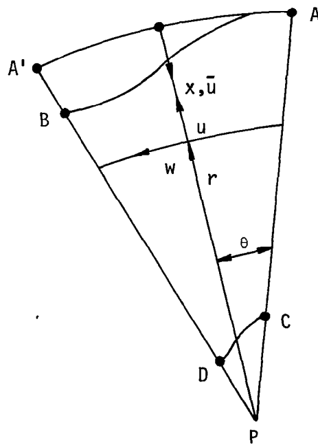
Figure 4. Notation for conical section ABDC and the coordinate system in the developed plane.
