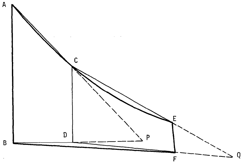
Figure 3. Representation of the wing by conical sections.
