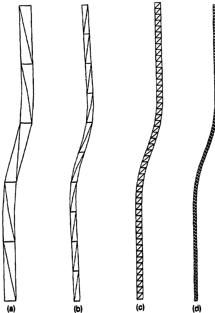
Fig. 3. Incremental displacement patterns at a residual load level of \sigma_{xy}/\bar{\sigma} = 0.28 . (a) 10 elements; (b) 20 elements; (c) 100 elements; (d) 200 elements.
