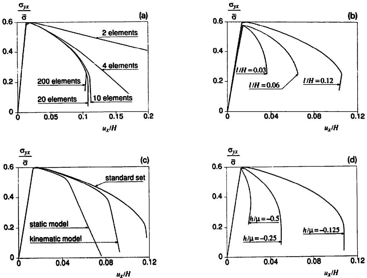
Fig. 4. Load–displacement diagram for shear layer. Results for a Cosserat continuum with strain softening. (a) The effect of mesh refinement; (b) the role of the characteristic length l ; (c) influence of the parameter set (a_1, a_2, a_3) ; (d) influence of the softening modulus h .
