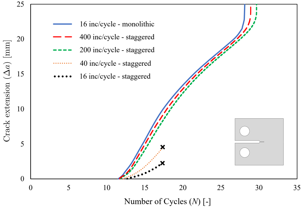
Figure 10: Fatigue crack growth in a CT specimen: influence of the solution scheme. Crack extension \Delta a versus number of cycles N as predicted with a staggered and a monolithic quasi-Newton scheme. The phase field AT2 model has been used.
