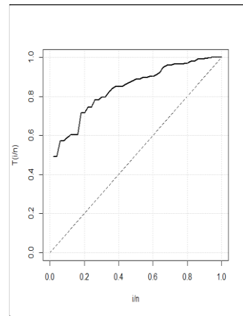
Figure 7: TTT plot for data set III.
