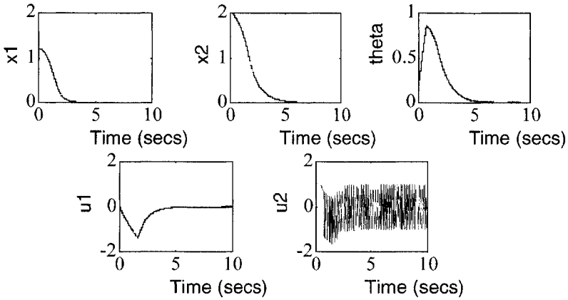
FIGURE 4 Stabilization of (12) using (14) with k_{i=1,2}(\cdot) = 1 .
