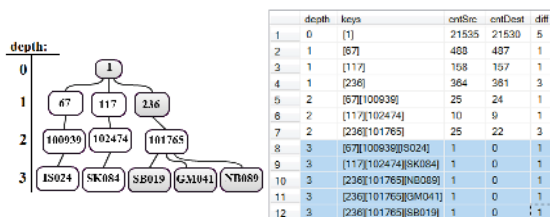
Fig. 7. The full drill down tree for Table 5 and the corresponding result table
