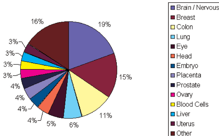
Figure 4. A summary of the tissue sources from which the non-linear spliced ESTs for 170 human genes were derived. Tissue source information was obtained from the GenBank records of the EST sequences.
