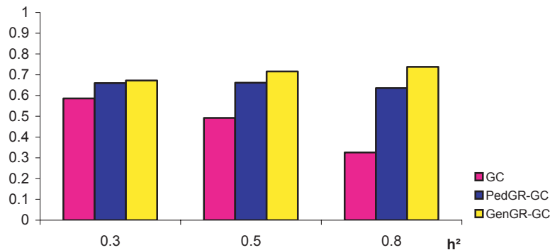
Figure 2. Type 1 error (A) and power (B) to achieve 5% genome-wide significance at the truly associated SNP in a study of 695 ERF people genotyped for 5524 autosomal SNPs. doi:10.1371/journal.pone.0001274.g002
