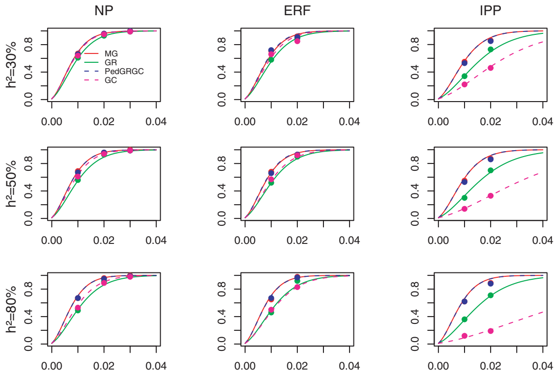
Figure 1. Power of MG (red line), GRAMMAR (green line), PedGR-GC (blue dashed line), and GC (pink dashed line) to detect association under different heritability models and pedigree structures. The three rows show the power under different heritability models (from 30% to 80%) and the three columns show power achieved in different pedigrees namely nuclear pedigrees (NP), Erasmus Rucphen Family (ERF), and idealized pig population (IPP). The y-axis of each panel shows power while the x-axis shows the proportion of variance explained by the QTL under study. The red (for MG), green (for GRAMMAR), blue (for PedGR-GC), and pink (for GC) circles show the empirical power estimates. The power estimates are based on \alpha=0.01 . The empirical power estimates are based on 1000 simulations for NP, and IPP, and 100 simulations for ERF. doi:10.1371/journal.pone.0001274.g001
