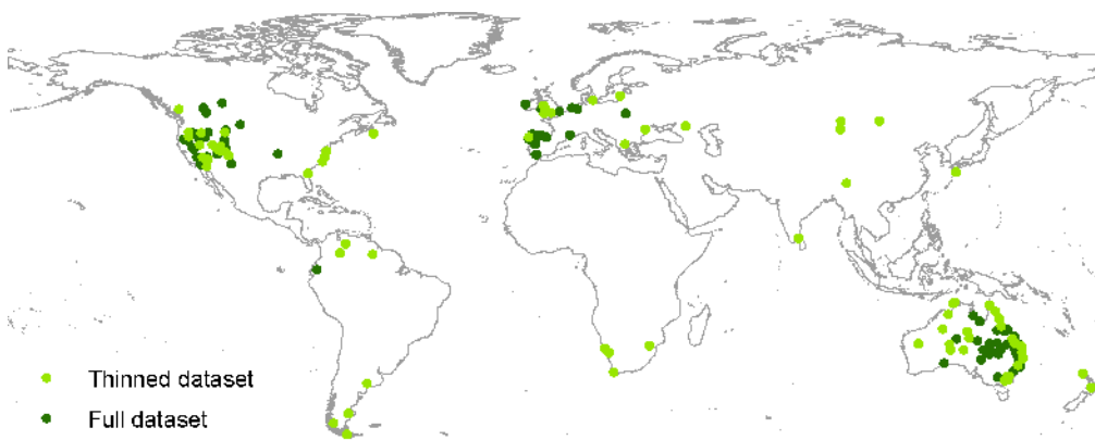
Fig 2. Current distribution of wild-living horses ( E. ferus ). The dots indicate the 186 populations of recent wild-living E. ferus identified in this study. Light green, included by the OccurrenceThinner procedure (n = 76); and dark green, excluded (n = 110) (see the text for further details).
