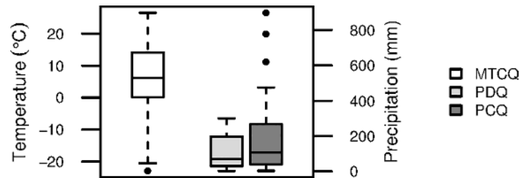
Fig 3. Analysis of feral horse occurrences using species distribution modelling. MAXENT species distribution modelling of the selected wild-living horse ( E. ferus ) localities ( n = 76 ) worldwide using climatic predictor variables. (A) Test gain jackknife evaluation of the relative importance of all variables considered; (B) Test gain jackknife evaluation of the relative importance of the three selected variables; and (C) Estimated response curves (showing the probability of presence using the logistic output from MAXENT). For acronyms, see Table 1 .
