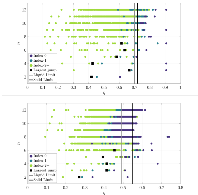
FIG. 9: The largest discontinuous jumps (black squares) observed in Figs. 7 (top) and 8 (bottom) along with the packing fractions of all known critical points, colored by their indices (index-0 in purple, index-1 in blue, all others in green).
