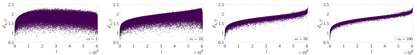
FIG. 11: The same configurations as in Fig. 10 are sorted by the approximate values of d_{\Lambda/\tau}[\mathbf{x}, S(\mathbf{y})] for m = 1, 10, 50, and 100 and are plotted with the true values of d_{\Lambda/\tau}[\mathbf{x}, S(\mathbf{y})] on the vertical axis.
