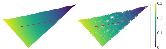
FIG. 4: The quotient space \Lambda(2)/\{\mathcal{T}, \mathcal{P}, \mathcal{L}\} of two points on T^2 represented as an \alpha -complex (left) and a graph (right), with color indicating the value of the tautological function. The red path connecting two points is a straight line on the left, but is slightly longer on the right.
