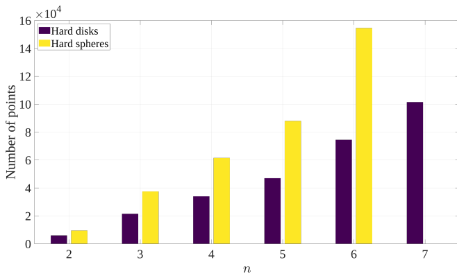
FIG. 3: Number of points used in the graph representations for hard disks and spheres.
