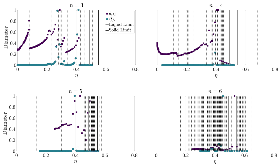
FIG. 8: Diffusion diameters and \epsilon -mixing times of the spaces \Gamma/\{\mathcal{T} \cup \mathcal{P} \cup \mathcal{L}\} for n = 3 \dots 6 hard spheres as functions of packing fraction. Dashed lines shows the packing fractions of the critical points.
