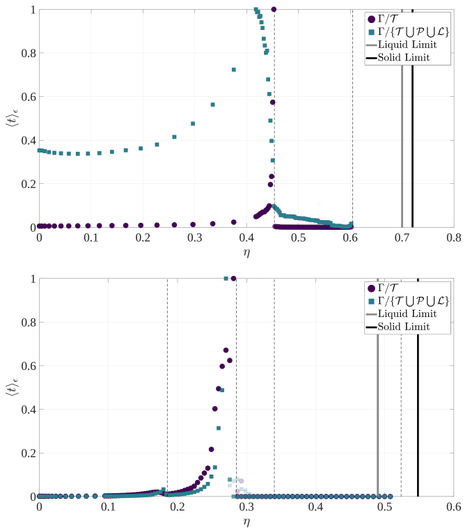
FIG. 6: \epsilon -mixing times of the quotient spaces \Gamma(2, \eta)/\mathcal{T} and \Gamma(2, \eta)/\{\mathcal{T} \cup \mathcal{P} \cup \mathcal{L}\} for hard disks (top) and hard spheres (bottom). Dashed lines represent the packing fractions of the critical points.
