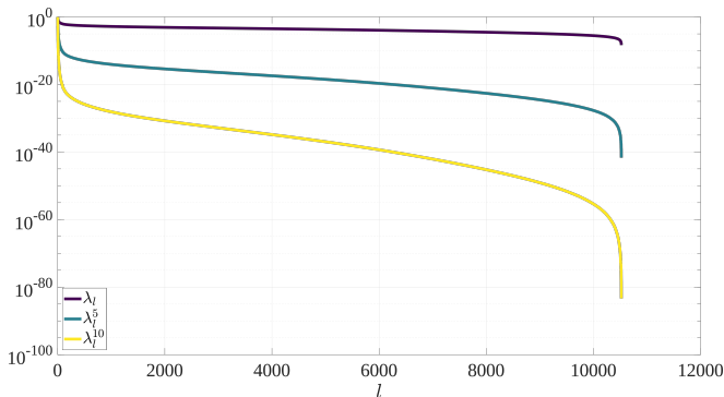
FIG. 12: The t th powers of the eigenvalues of \mathbf{P} for \Lambda(4)/\{\mathcal{T} \cup \mathcal{P} \cup \mathcal{L}\} at times t = 1, 5, and 10 . The values generally decay rapidly, and are often numerically indistinguishable from zero for sufficiently large t .
