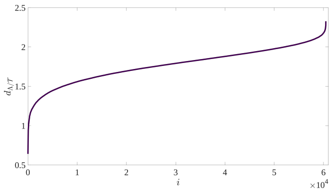
FIG. 10: The sorted true distances d_{\Lambda/\mathcal{T}} calculated for a fixed generic configuration and the 7! \times 12 symmetric versions of a second generic configuration for 7 hard disks.
