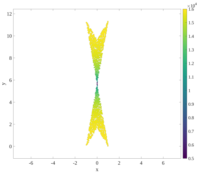
FIG. 13: Individual mixing times t_{\epsilon}(\mathbf{q}_0) of the example system shown in Fig. 1. The average mixing time \langle t \rangle_{\epsilon} is around 15\,000 .
