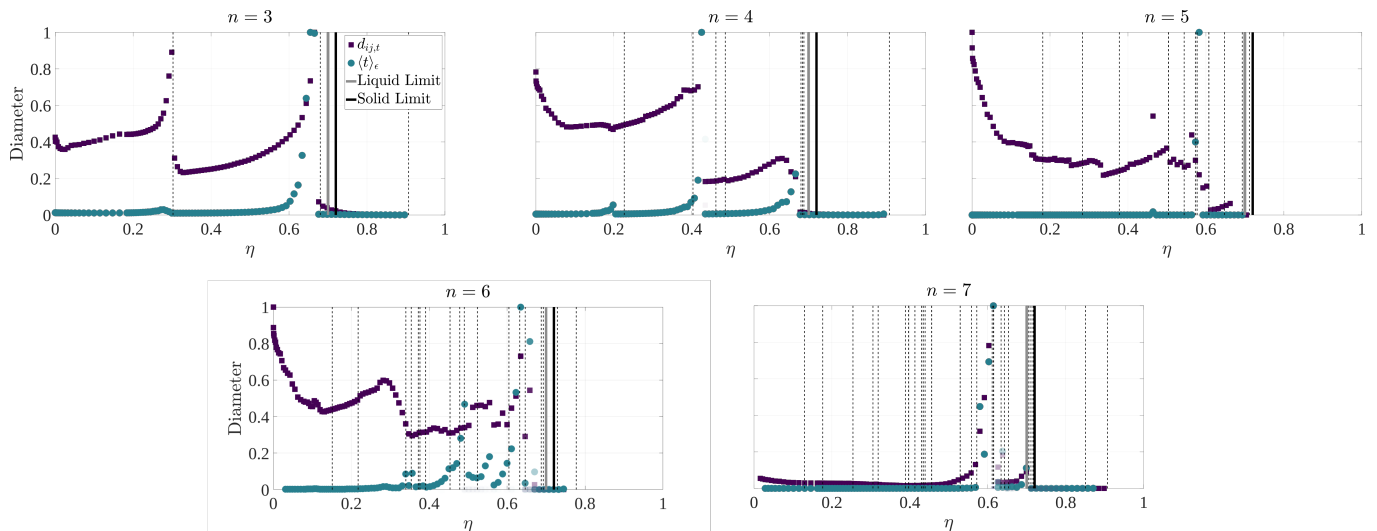
FIG. 7: Diffusion diameters and \epsilon -mixing times of the spaces \Gamma/\{\mathcal{T} \cup \mathcal{P} \cup \mathcal{L}\} for n = 3 \dots 7 hard disks as functions of packing fraction. Dashed lines shows the packing fractions of the critical points.
