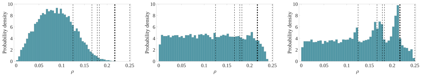
FIG. 5: Distributions of tautological function values for point clouds on \Lambda(4) sampled by three different procedures, with the dashed lines indicating the radii of previously-identified critical points. Sampling points uniformly gives the distribution on the left. The distribution in the middle uses importance sampling and is more uniform. The distribution on the right is for a point cloud that both uses importance sampling and samples additional points in the neighborhoods of the critical points.
