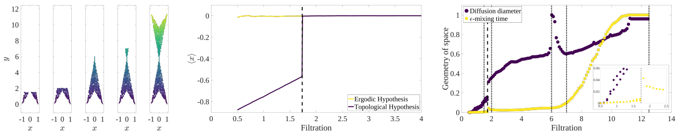
FIG. 1: The left panel shows the evolution of a model configuration space with points colored by their y -coordinate. The filtration value is an upper bound for the y -coordinate of any point on the system’s trajectory. The middle panel shows the average x -coordinate \langle x \rangle calculated using the ergodic hypothesis and the topological hypothesis as a function of filtration value, assuming that the system starts at the lower left corner of the configuration space. The right panel shows the diffusion diameter and \epsilon -mixing time of the configuration space as functions of filtration value and that they are sensitive to changes in the configuration space geometry. The diffusion diameter, but not the mixing time, is also sensitive to the bottleneck. The five dotted lines show the filtration values used in the left panel.
