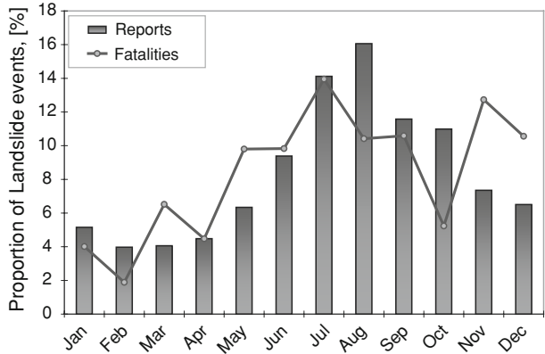
Fig. 3 Combined distribution of landslide reports and fatalities for 2003, 2007, and 2008 shown as a proportion of the total per month
