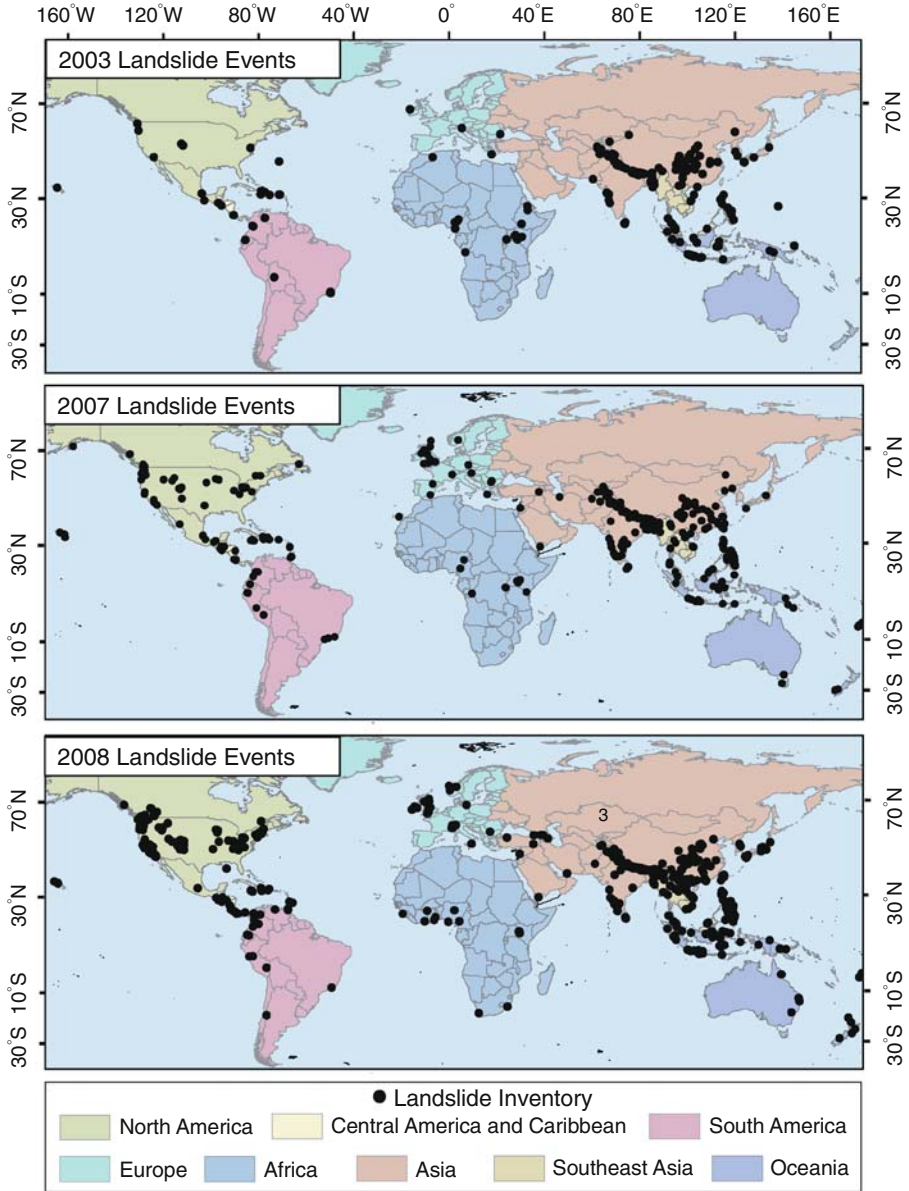
Fig. 2 Maps of landslide locations for the 3 years of the landslide catalog, shown according to geographic region
