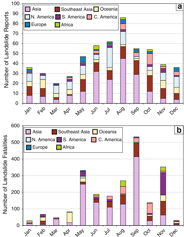
Fig. 5 Total number of landslide reports (a) and fatalities (b) for 2008 as a function of month and region
