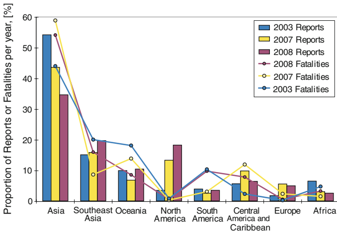
Fig. 4 Proportion of landslide reports and fatalities by region for the 2003, 2007, and 2008
