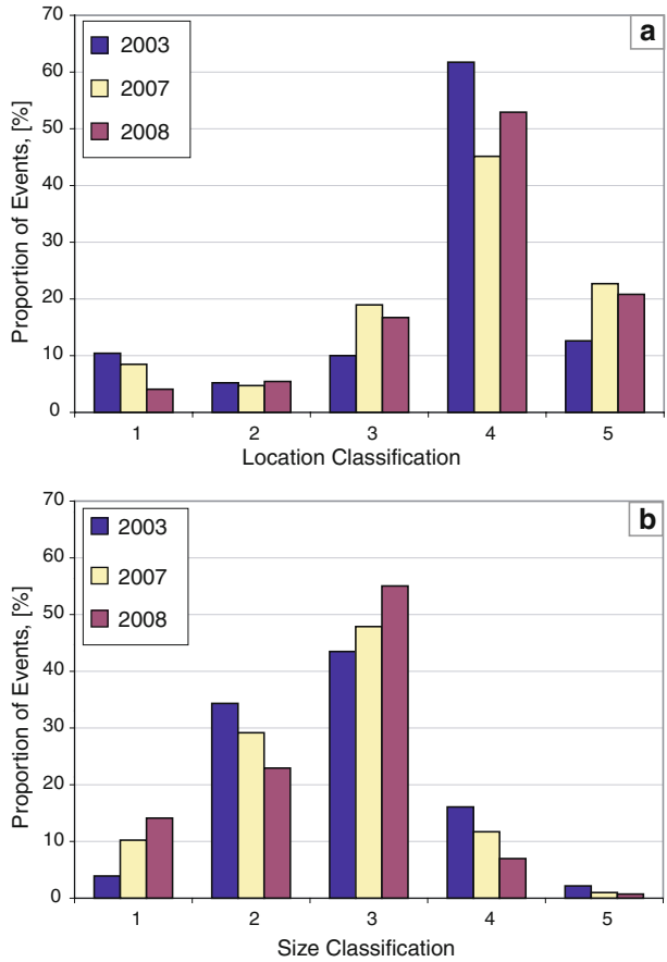
Fig. 1 (a) Location classification and (b) size classification distribution for the 3 years of the landslide catalog
