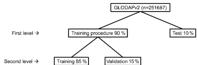
Figure 2. Division of the data for the training of the network and its testing. The percentages in each level are relative to the previous one.
