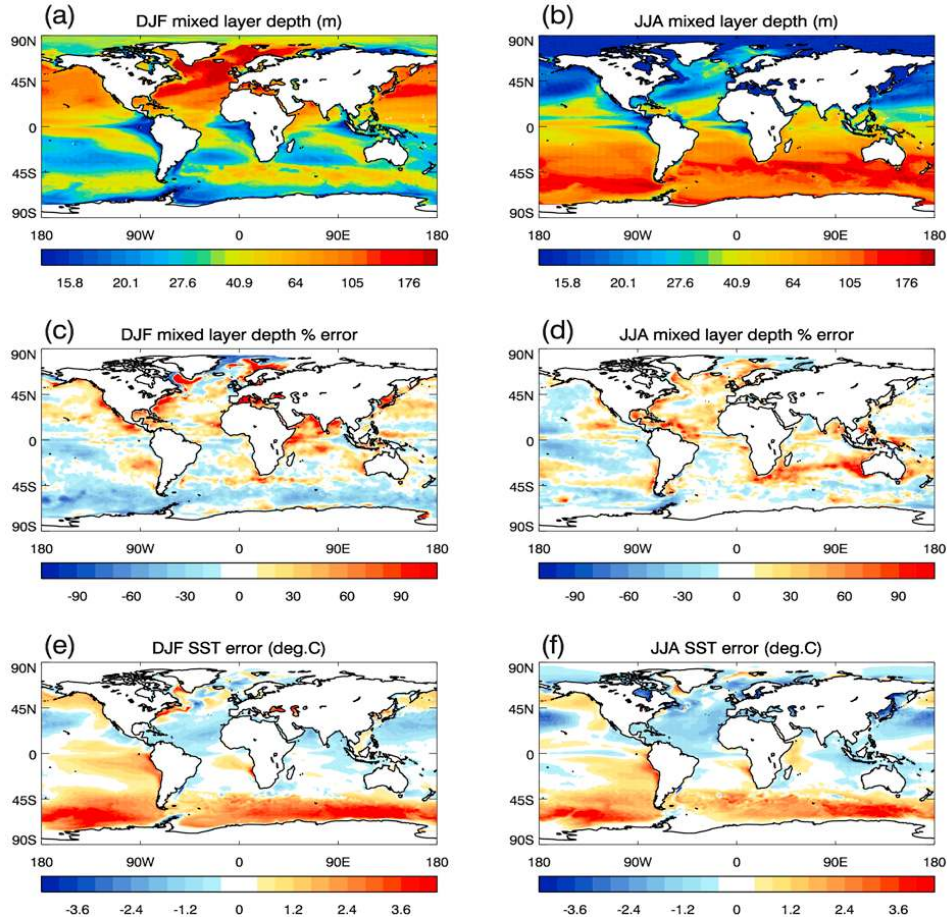
Figure 1. Seasonal variation in the OSBL depth computed with HadGEM3 averaged over 20 years and comparisons with Argo float measurements reported in de Boyer Montégut et al. [2004] updated to include data up to 2008: (a) computed depth DJF, (b) computed depth JJA, (c) percentage error between simulated and measured depths for DJF, (d) percentage error between simulated and measured depths for JJA. Corresponding errors in sea surface temperature: (e) DJF, (f) JJA.
