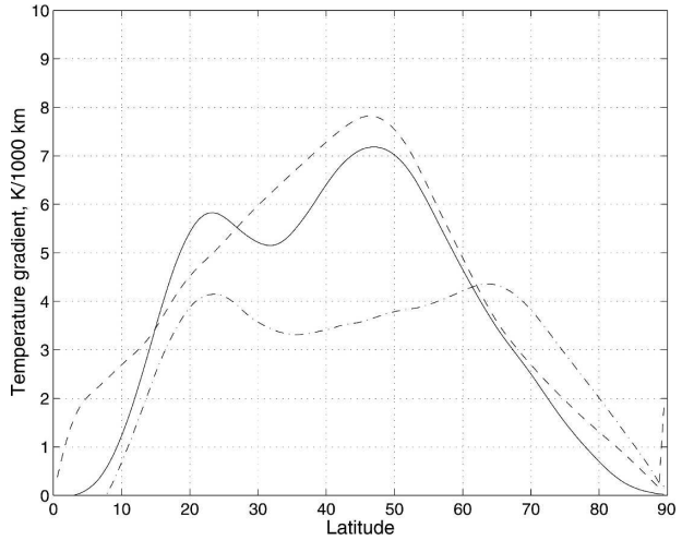
FIG. 10. Meridional temperature gradients at 630 hPa, in \text{K} (1000 \text{ km})^{-1} (solid = control case, dashed = dry limit, dash-dot = 10X case).
