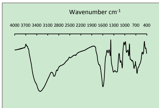
Figure 3. FT-IR of carob leaf extract
