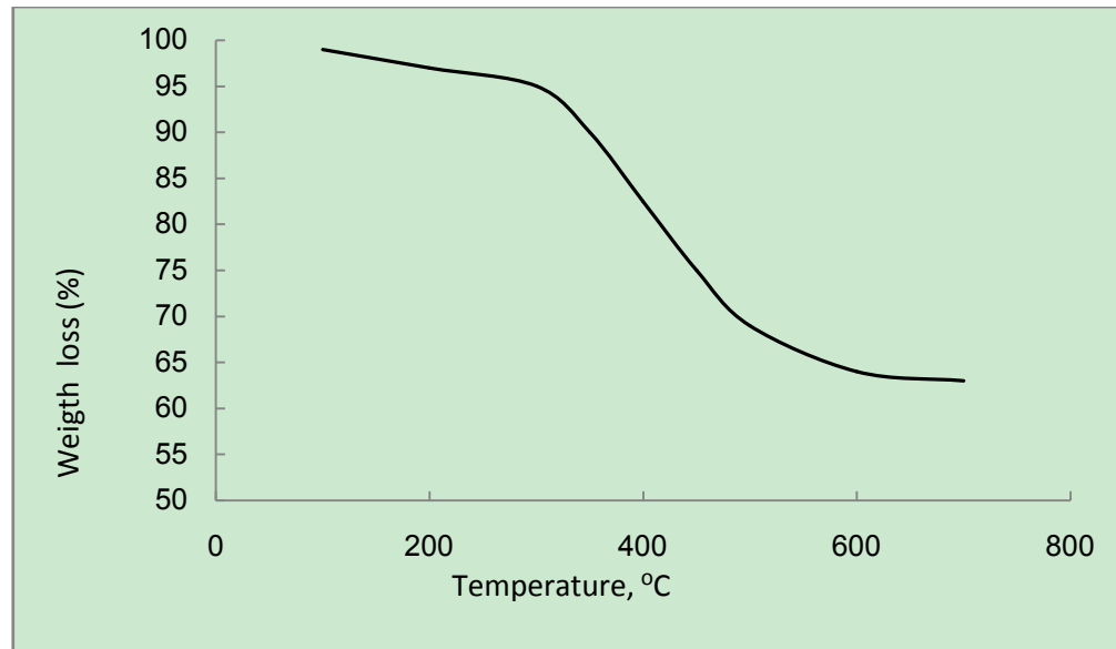
Figure 8. TGA curve of magnetite nanoparticles
