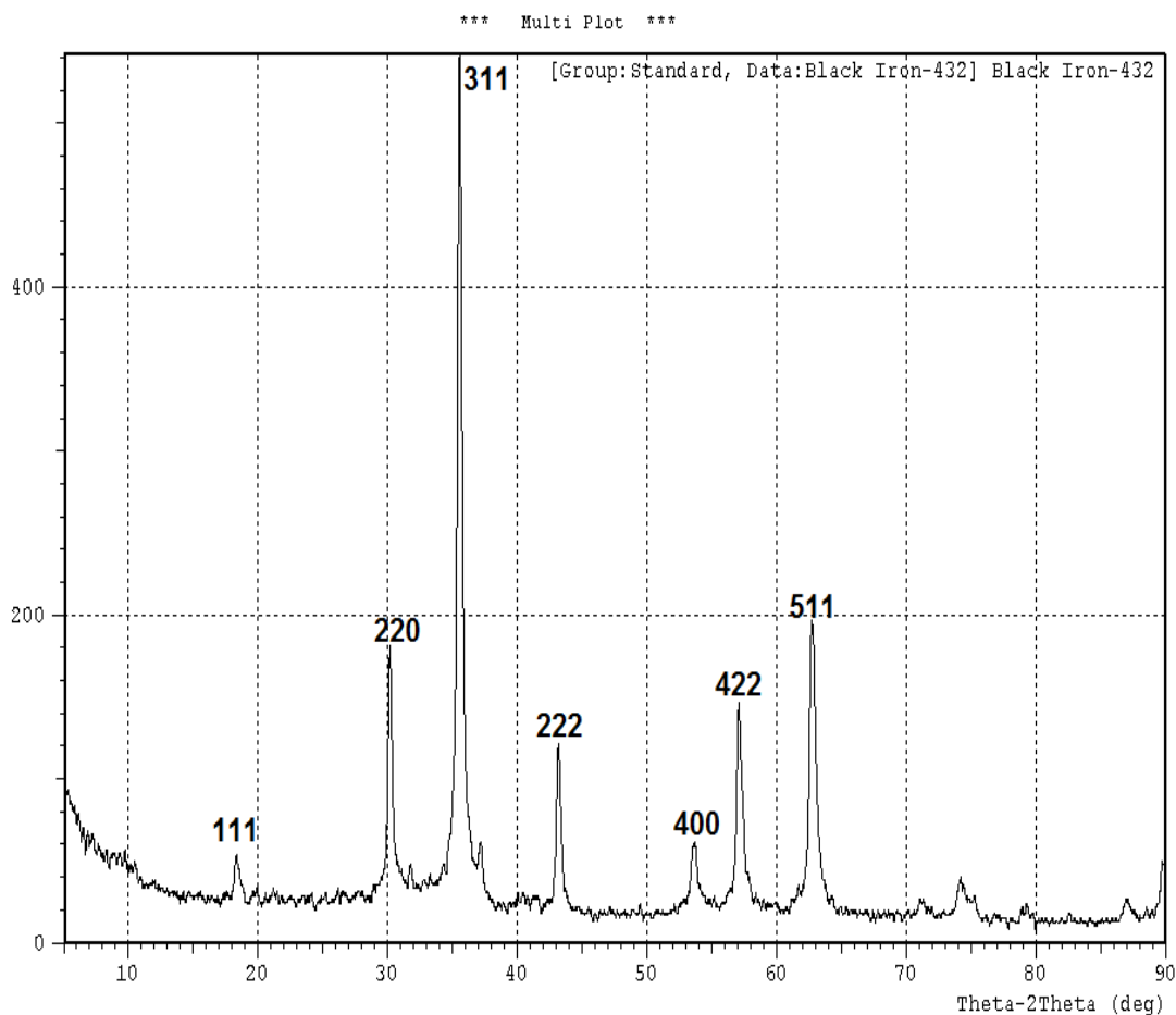
Figure 2. XRD of synthesized magnetite nanoparticles
