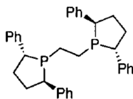
(R,R) -Ph-BPE
