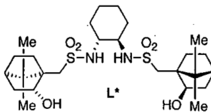
Figure 32. Asymmetric addition of alkyl groups to ketones.
