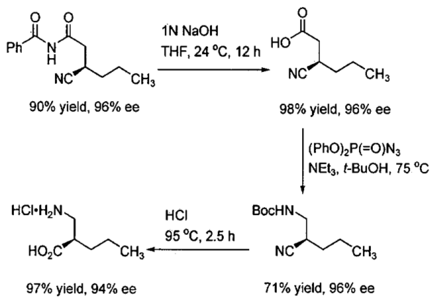
Figure 47. Synthesis of an enantioenriched \alpha -substituted- \beta -amino acid.
