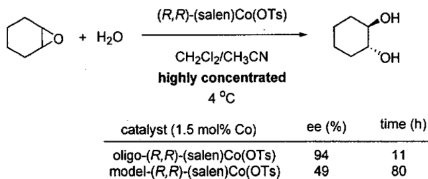
Figure 9. Comparison of the ARO of cyclohexene oxide with oligomeric and monomeric model catalysts from Figure 8.
