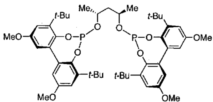
(2R,4R) -Chiraphite
