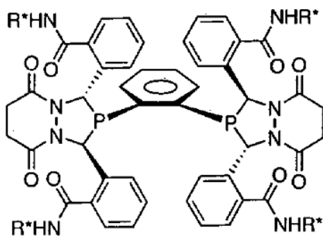
(2R,4R) -Chiraphite
