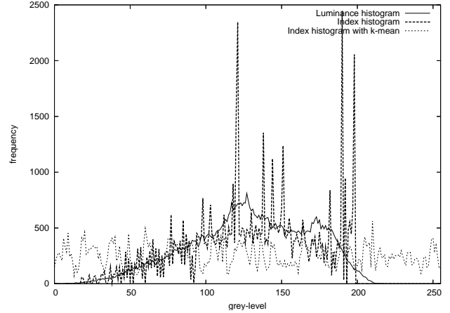
Fig. 2. Histograms.
