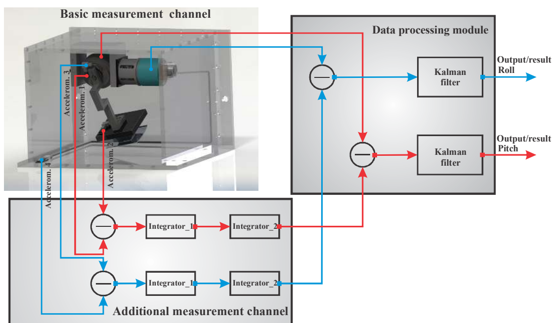
Fig.2. Block diagram of the measuring system.
