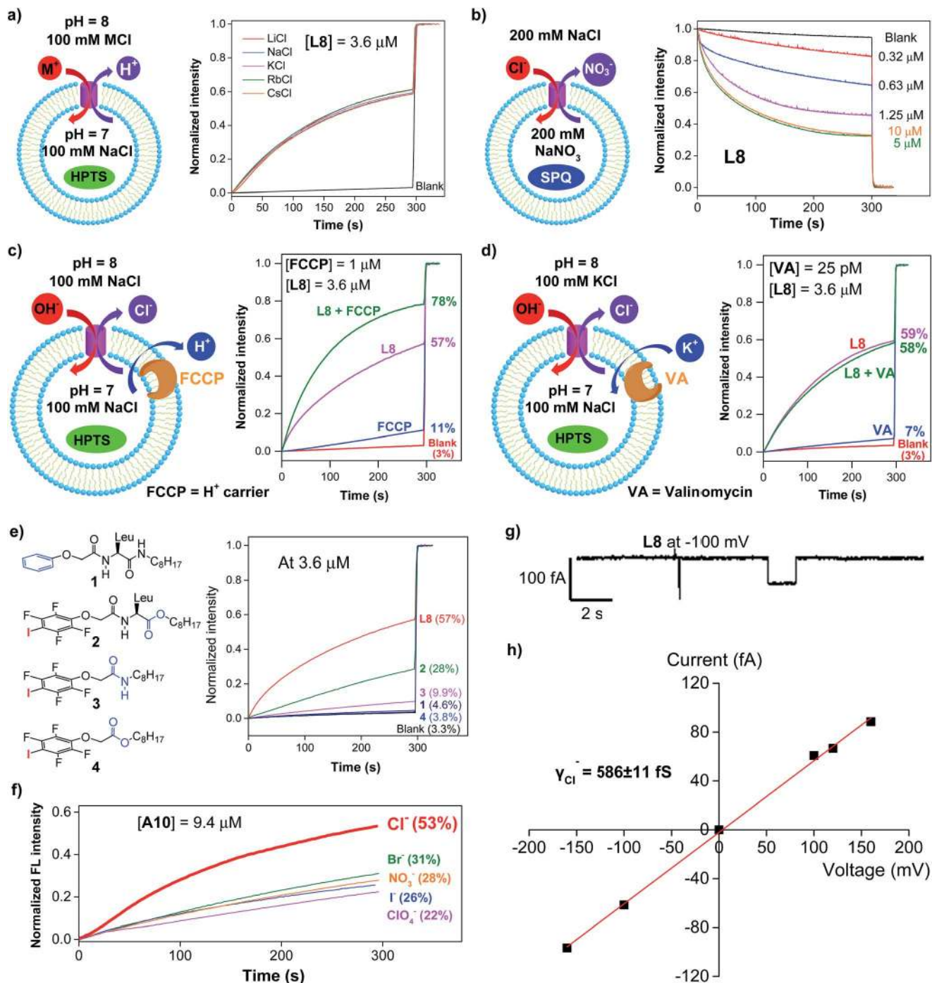
Fig. 3 (a) Transport selectivity of alkali metal ions by L8 (3.6 μM) obtained from the HPTS assay by varying the extravesicular MCl ( M^+ = \text{Li}^+, \text{Na}^+, \text{K}^+, \text{Rb}^+ and \text{Cs}^+ ). (b) Concentration-dependent changes in the fluorescence intensity of the chloride-sensitive SPQ dye ( \lambda_{\text{ex}} = 360 \text{ nm} , \lambda_{\text{em}} = 430 \text{ nm} ) after the addition of L8 at different concentrations. Inside LUV: 200 mM \text{NaNO}_3 and 0.5 mM SPQ. Outside LUV: 200 mM \text{NaCl} . (c) Ion transport activities of L8 (3.6 μM) determined in the absence or presence of proton transporter FCCP (1 μM), indicating a preferential transport of \text{Cl}^- over \text{H}^+ . (d) Ion transport activities of L8 (3.6 μM) determined in the absence or presence of a potassium carrier, valinomycin (VA, 25 pM), indicating a preferential transport of \text{Cl}^- over \text{OH}^- . (e) Ion transport activities of four control compounds 1–4 at 3.6 μM, suggesting a critical role of halogen bonds in mediating the transport of \text{Cl}^- and \text{OH}^- . (f) Anion selectivity assayed for A10 (For L8 and L10, see Fig. S10†). (g) Single current trace of L8 recorded at -100 mV with symmetric baths (cis chamber = trans chamber = 1 M KCl). (h) I - V curve for obtaining the \text{Cl}^- conductance ( \gamma_{\text{Cl}^-} ) of L8. All the data were averaged over two measurements.
