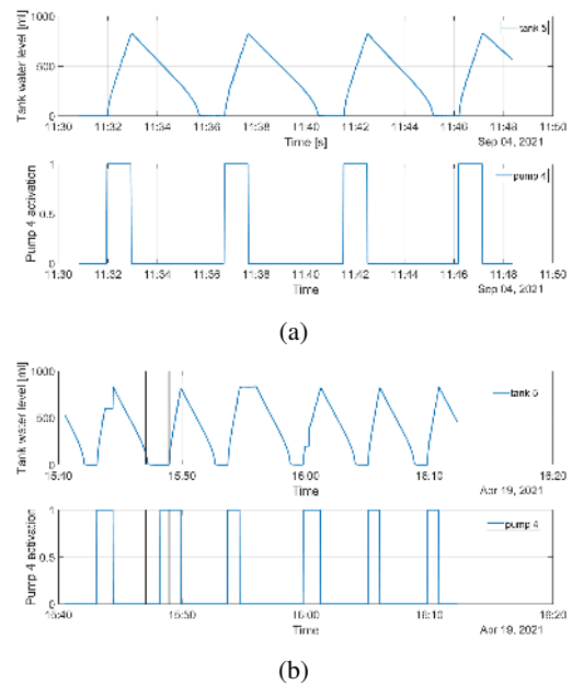
FIGURE 8: Effects of a physical attack against P_4^r on the physical process (Scenario 2.6). The attack causes the breakdown of P_4^r , which stops water flow towards T_5^r . (a) shows the normal scenario, while (b) the effect of the attack. Black lines indicate the start and the end of the physical attack.
