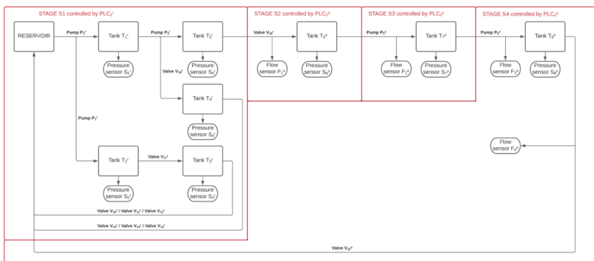
FIGURE 3: WDT physical process divided into 4 stages: the first is controlled by the real PLC, PLC_1^r , while the remaining ones are controlled by the simulated PLCs, PLC_2^s , PLC_3^s and PLC_4^s
