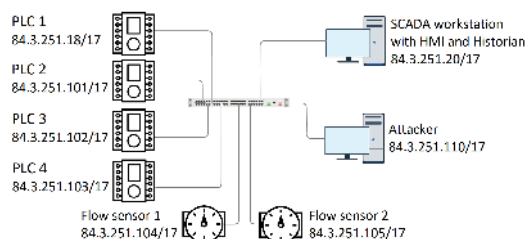
FIGURE 5: SCADA network
