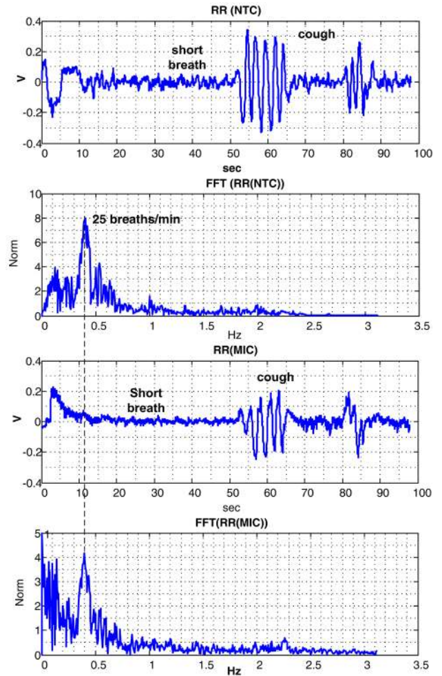
Figure 9: Real signal with noise and cough. The dominate RR is detected from FFT Spectrum.
