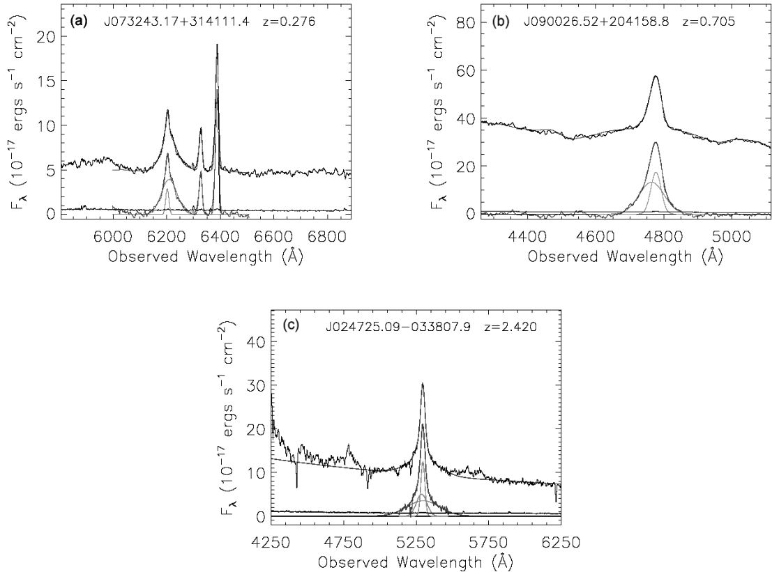
Fig. 21.— Examples of broad emission line fits. (a): H\beta ; (b): Mg\text{ II} ; (c): C\text{ IV} . For each panel, the upper black line shows the original SED. The lower blue line shows the continuum and Fe subtracted SED. The upper magenta line shows the full fits; the lower magenta line shows the fits for the emission lines; the gray lines show the flux density errors; the green lines show the broad Gaussian components, while the red lines show the narrow Gaussian components.
