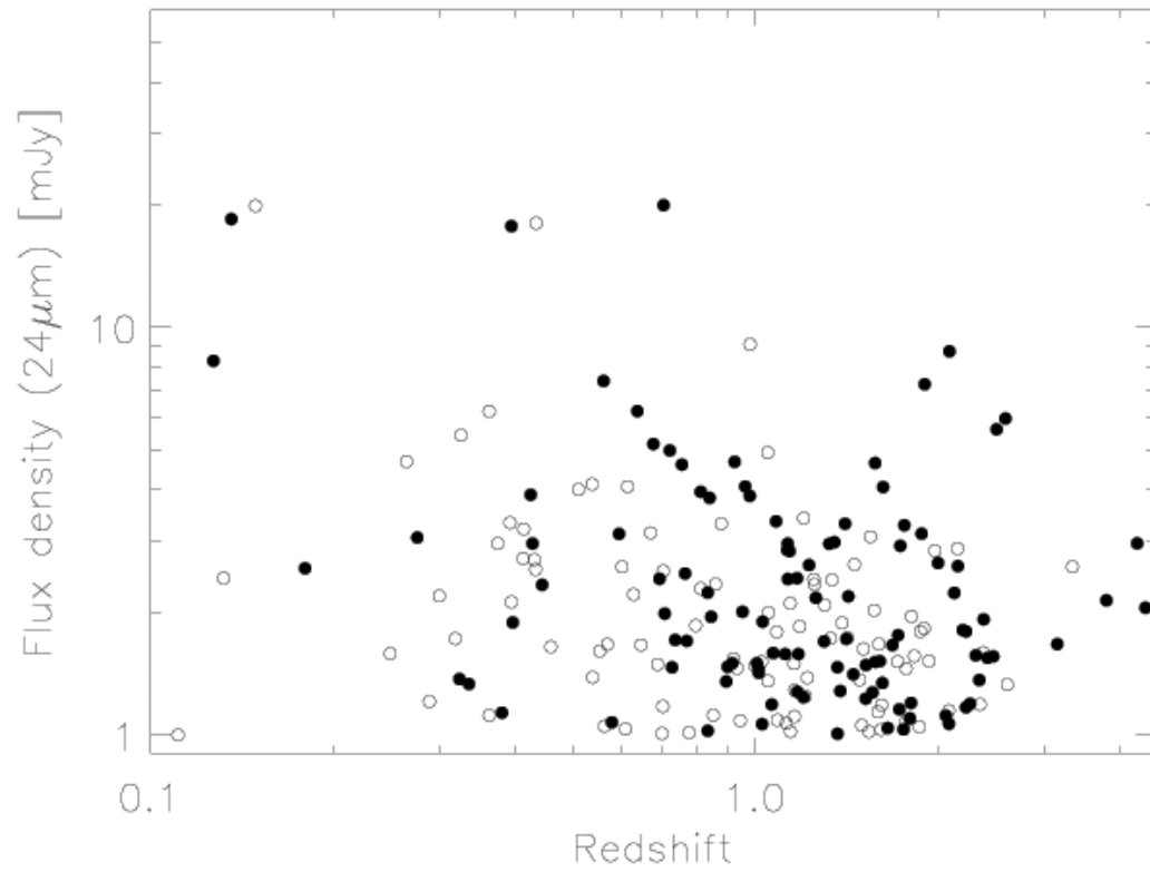
Fig. 2.— 24 \mu\text{m} flux density versus redshift for Type-1 AGNs with 24 \mu\text{m} flux density > 1 \text{ mJy} in our survey area. The filled circles show Herschel -detected Type-1 AGNs. The unfilled circles show Herschel -non-detected Type-1 AGNs.
