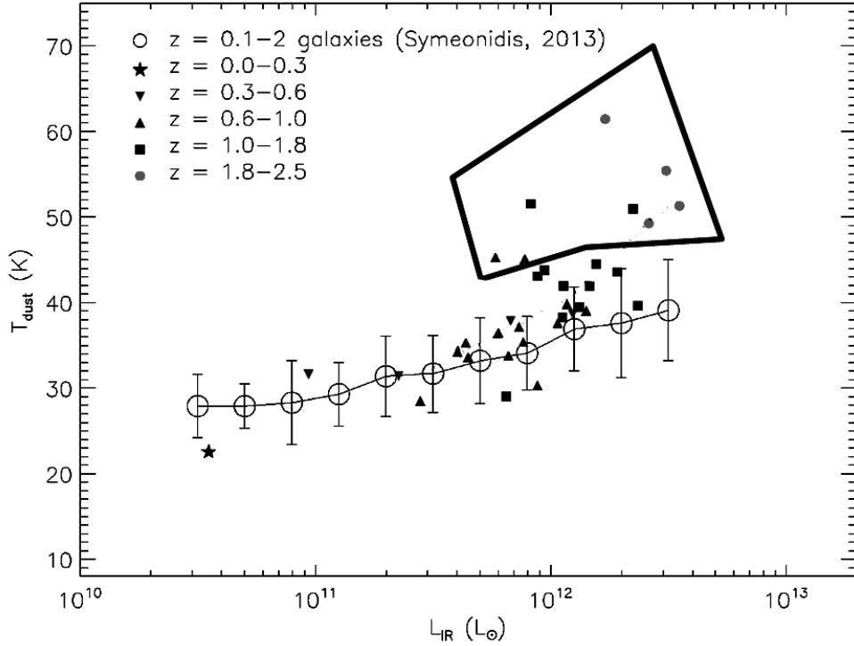
Fig. 7.— The FIR dust temperature versus total infrared luminosity (rest-frame 8 \mu\text{m}-1000 \mu\text{m} ). The big circles (blue) show the L-T relation of star-forming galaxies ( z=0.1-2 ) derived from HERMES and PEP data in COSMOS, GOODS-S and GOODS-N fields (Symeonidis et al., 2013). The error bars show the 1-sigma scatter of the L-T relation. The blue irregular polygon encloses the sources with strong warm infrared components. The remaining sources are compatible with the L-T relation, particularly if one allows for modest warm components in a few of them.
