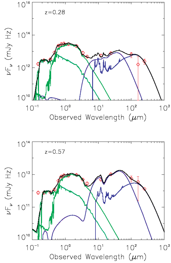
Fig. 14.— The average SEDs for Type-2 AGNs with no formal FIR detections in our sample in two discrete redshift bins: z = 0.0-0.4 (upper, 14 sources), and 0.4-0.8 (lower, 13 sources). Symbols and line colors are the same as in Figure 13.
