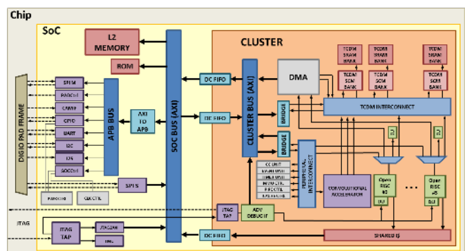
Fig. 1: Mia Wallace SoC architecture
