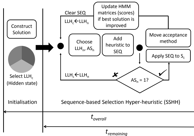
Figure 4: A sequence-based selection hyper-heuristic utilising HMM; where LLH_c and LLH_n are the current and next selected low level heuristics, respectively, and AS_n is the next selected sequence-based acceptance strategy
