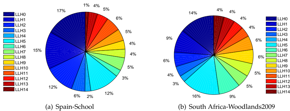
Figure 8: Average utilisation rate of each low level heuristic considering only invocations that generated improvement on the best-of-run solution and AS=1 & 2 from 10 runs using SSHH while solving Spain-School and South Africa-Woodlands2009 instances
