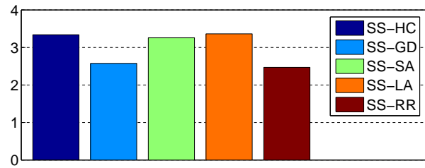
Figure 5: Comparisons of the different move acceptance methods when combined with the sequence-based selection method. The vertical axis shows the score values using ITC 2011 ranking strategy over 10 runs from eight instances
