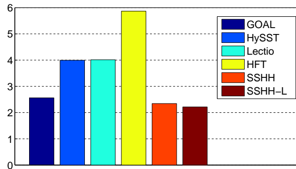
Figure 13: Comparisons of ITC solvers, SSHH and SSHH-L based on ITC 2011 ranking strategy over 10 runs for each ITC 2011 instances
