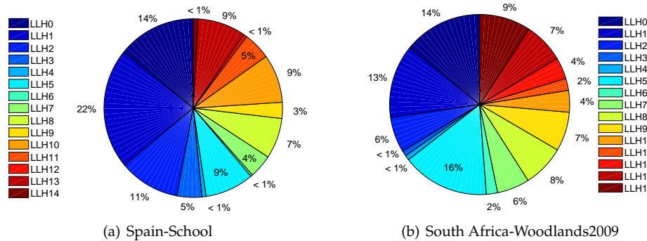
Figure 10: Average utilisation rate of each low level heuristic considering only invocations that generated improvement on the best-of-run solution and AS=1 & 2 from 10 runs using SSHH-L while solving Spain-School and South Africa-Woodlands2009 instances
