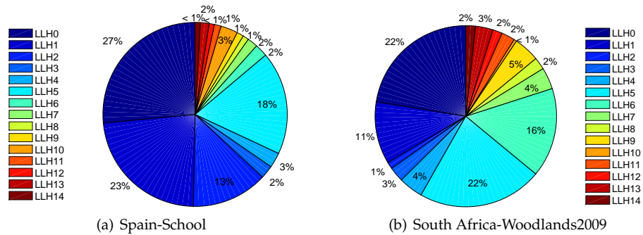
Figure 7: Average utilisation rate of each low level heuristic considering only invocations that generated improvement on the best-of-run solution and AS=1 from 10 runs using SSHH while solving Spain-School and South Africa-Woodlands2009 instances
