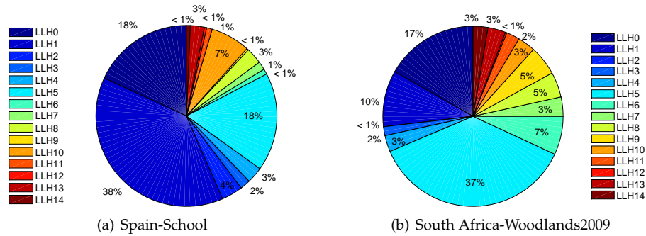
Figure 9: Average utilisation rate of each low level heuristic considering only invocations that generated improvement on the best-of-run solution and AS=1 from 10 runs using SSHH-L while solving Spain-School and South Africa-Woodlands2009 instances
