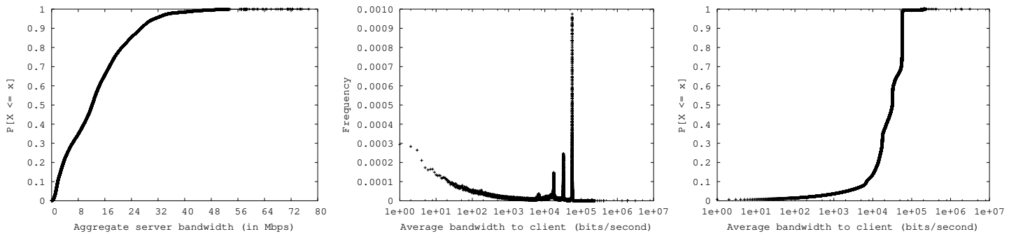
Figure 21. Cumulative distribution of aggregate b/w (left). Frequency (center) and cumulative (right) distribution of transfer b/w.
