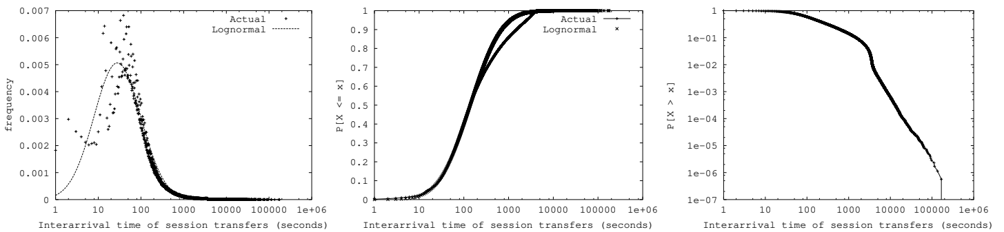
Figure 14. Marginal distribution of session transfer interarrivals: Frequency (left), cumulative (center), and CCDF (right)
