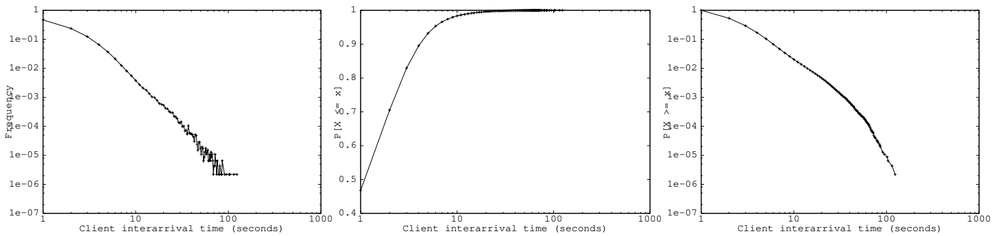
Figure 7. Interarrival times from a piece-wise-stationary Poisson process: Frequency (left), cumulative (center), and CCDF (right)
