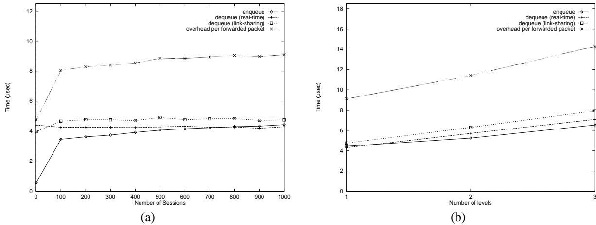
Fig. 13. (a) The overheads for a flat hierarchy with 1, 100, . . . , and 1000 sessions. (b) The overheads for a one-level, two-level, and three-level hierarchies, with each hierarchy having 1000 sessions.
